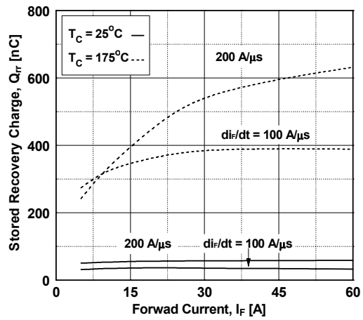
Figure 20. Stored Charge
