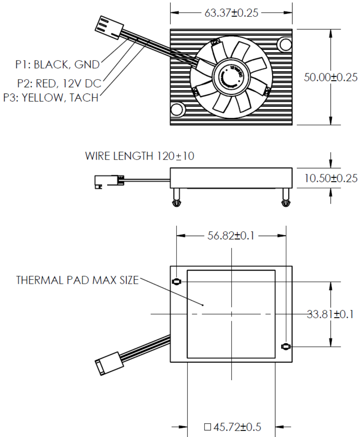
Figure 1: SZ12L Mechanical Drawings
