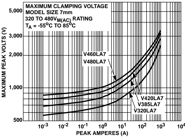
FIGURE 5. CLAMPING VOLTAGE FOR V320LA7 - V480LA7
