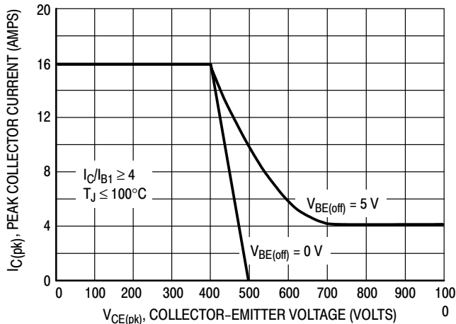
Figure 20. Maximum Reverse Biased Safe Operating Area
