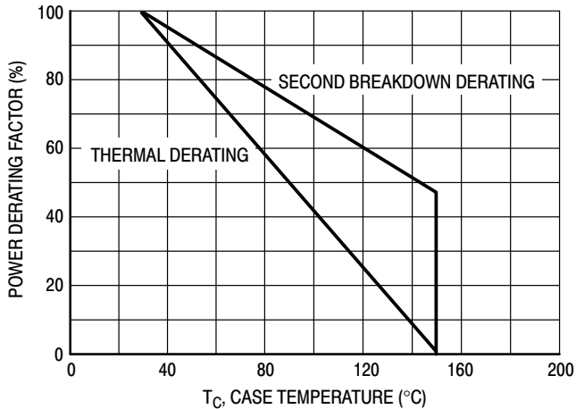
Figure 21. Power Derating
