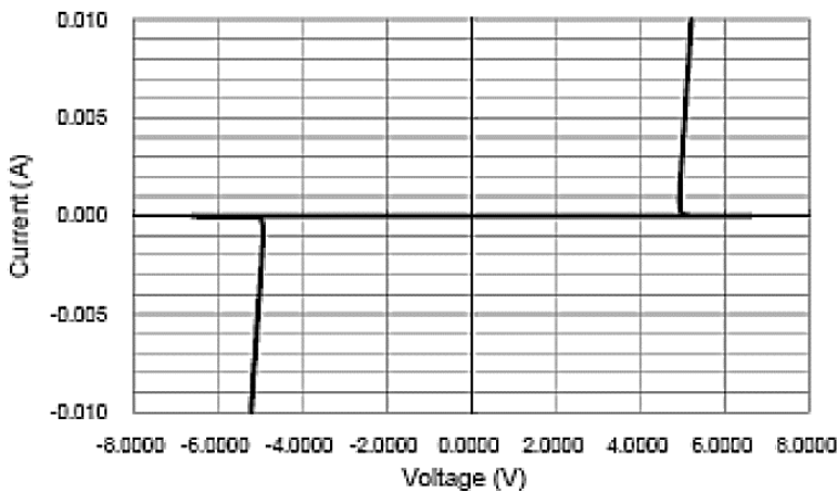
Fig 3 Voltage Sweeping
