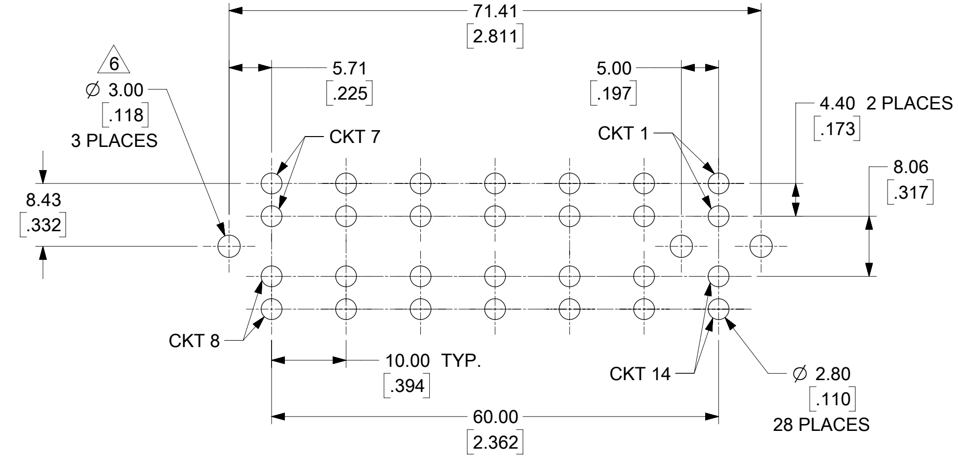
RECOMMENDED P.C. BOARD PLATED-THRU HOLE LAYOUT (RECOMMENDED PCB THICKNESS : 1.57mm)
