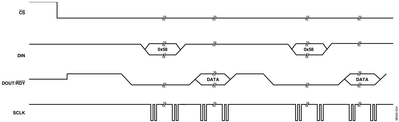
Figure 25. Continuous Conversion
