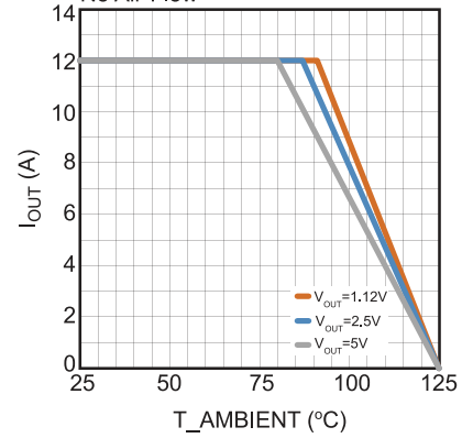
Thermal Derating V IN =12V, f S =800kHz, T J =125°C, No Air-Flow
