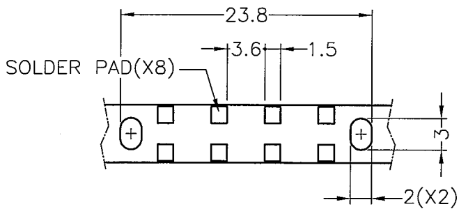
RECOMMEND PCB LAYOUT
