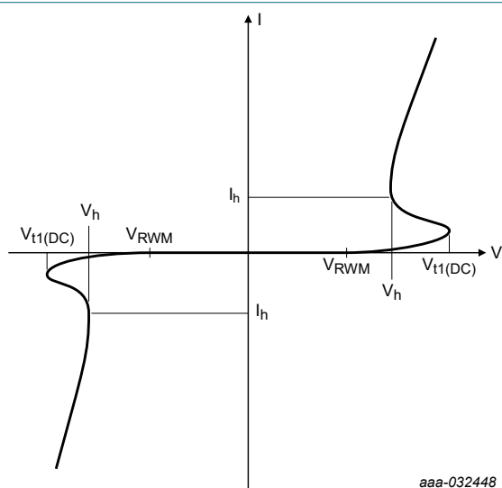
Fig. 3. Current forced I(V) characteristics for a bidirectional ESD protection device
