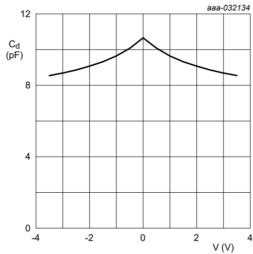
Fig. 9. Diode capacitance as a function of reverse voltage; typical values
