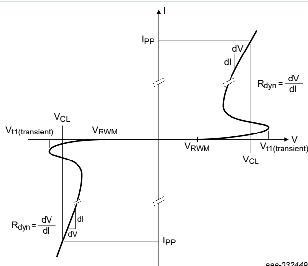
Fig. 4. Transient characteristics for a bidirectional ESD protection device
