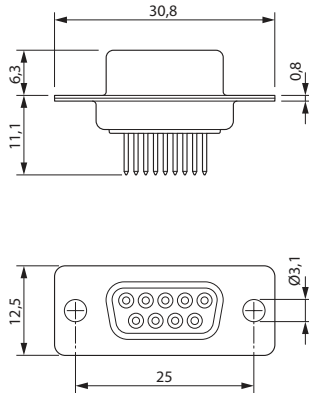
Dimensional drawing
