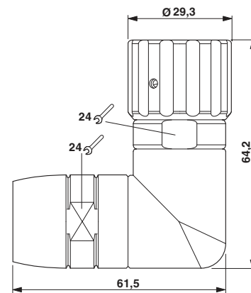
Dimensioned drawing
