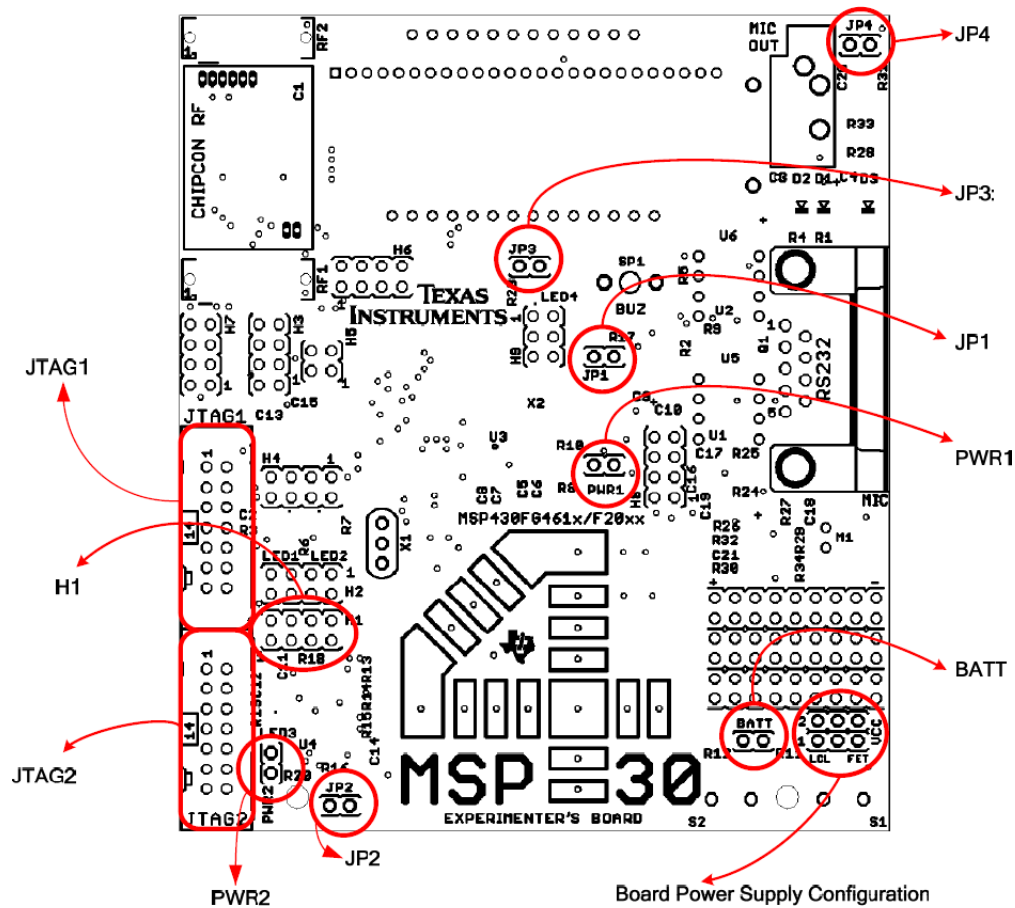
Figure 6. Jumper Locations
