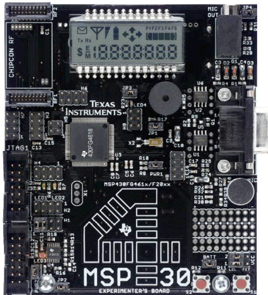
Figure 1. MSP430FG4618/F2013 Experimenter Board
