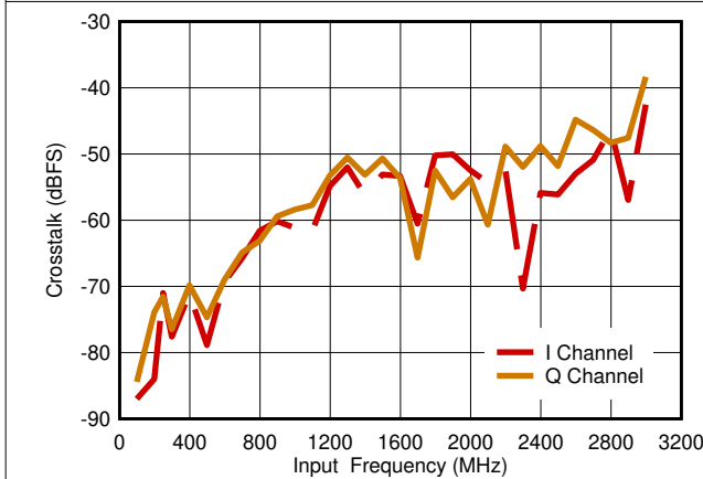
Figure 6-37. Cross Talk vs Input Frequency
