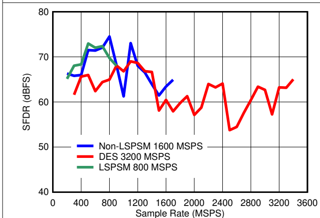
Figure 6-27. SFDR vs Sample Rate
