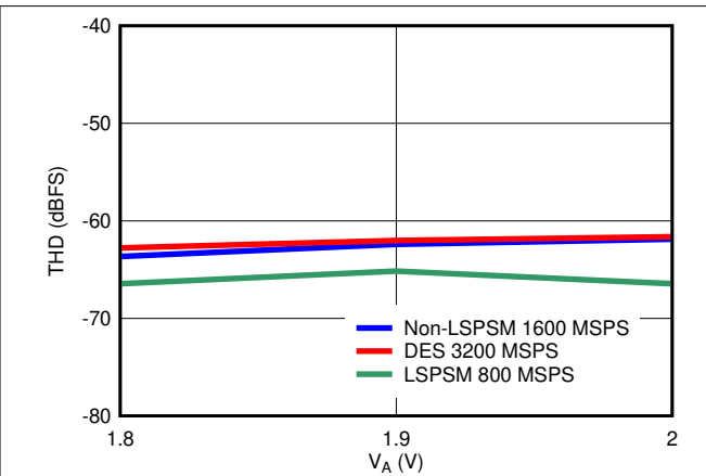
Figure 6-24. THD vs Supply Voltage
