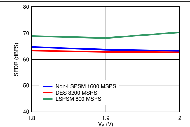
Figure 6-28. SFDR vs Supply Voltage
