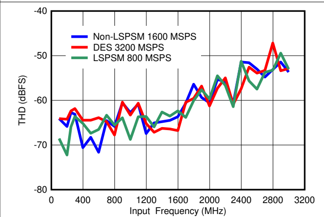
Figure 6-26. THD vs Input Frequency
