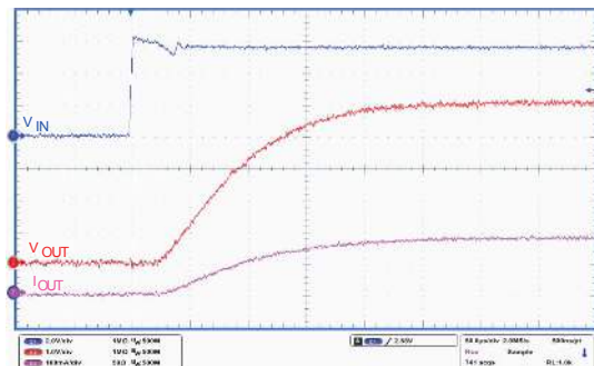
Figure 23. Turn-on time ( V_{OUT} = 5\text{ V} )
