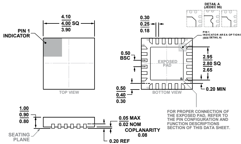
COMPLIANT TO JEDEC STANDARDS MO-220-VGGD-8. Figure 55. 24-Lead Lead Frame Chip Scale Package [LFCSP] 4 mm × 4 mm Body and 0.90 mm Package Height (HCP-24-2) Dimensions shown in millimeters
