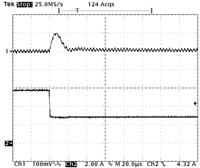
Fig-1.5V-7: Output voltage response for V_{out}=1.5V to negative load current step change from 6A to 3A with slew rate of -5A/\mu s at V_{in}=12V . C_o=47\mu F \times 2 ceramic. Top trace: output voltage (100mV/div.) Bottom trace: load current (2A/div.) Time scale: 20us/div.
