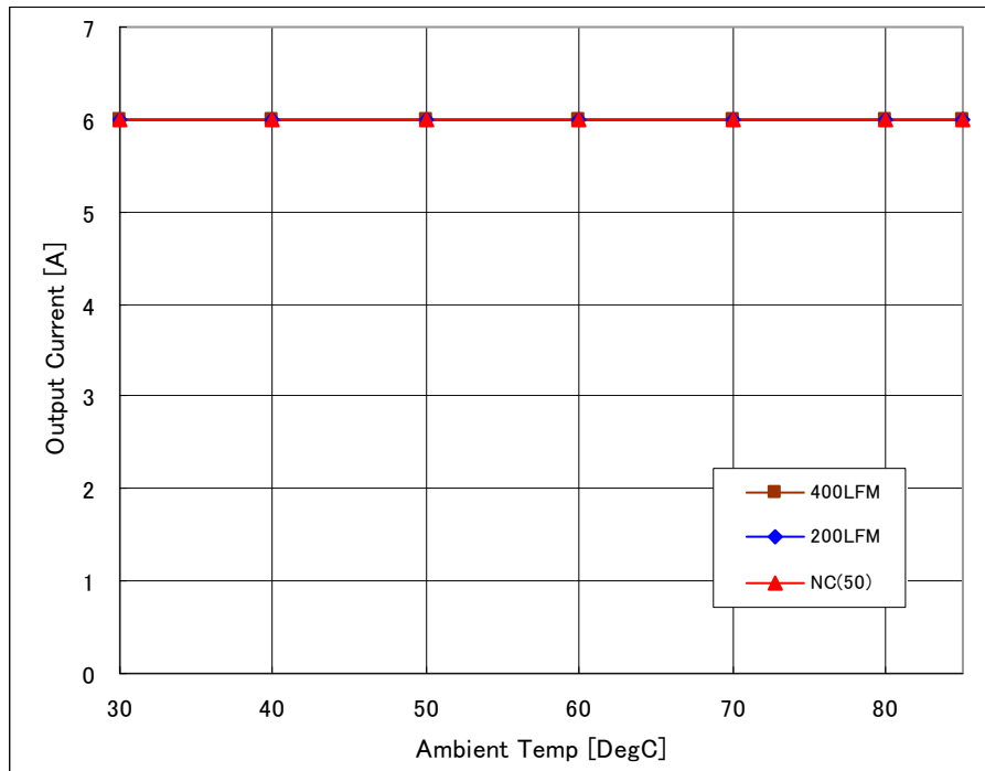
Fig-3.3V-1: Available load current vs. ambient temperature and airflow rates for Vout=3.3V with Vin=12V. Maximum component temperature ≤ 120°C
