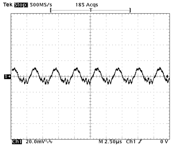
Fig-2.0V-5: Output voltage ripple (20mV/div.) for V_{out}=2.0V at full rated load current into a resistive load with external capacitance 47\mu F \times 2 ceramic + 1\mu F ceramic at V_{in}=12V .
