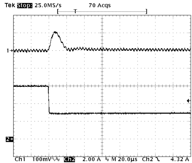
Fig-1.2V-7: Output voltage response for V_{out}=1.2V to negative load current step change from 6A to 3A with slew rate of -5A/us at V_{in}=12V . C_o=47\mu F \times 2 ceramic. Top trace: output voltage (100mV/div.) Bottom trace: load current (2A/div.) Time scale: 20us/div.
