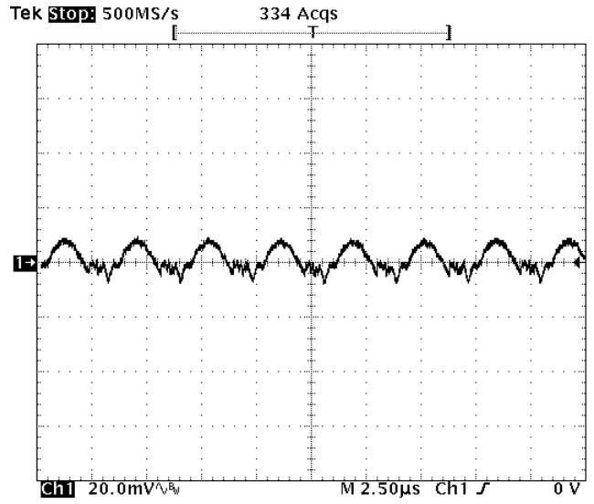
Fig-1.2V-5: Output voltage ripple (20mV/div.) for V_{out}=1.2V at full rated load current into a resistive load with external capacitance 47\mu F \times 2 ceramic + 1uF ceramic at V_{in}=12V . Time scale: 2.5 us/div
