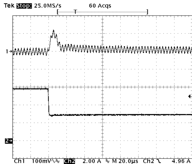
Fig-5.0V-7: Output voltage response for V_{out}=5.0V to negative load current step change from 6A to 3A with slew rate of -5A/\mu s at V_{in}=12V . C_o=47\mu F \times 2 ceramic. Top trace: output voltage (100mV/div.) Bottom trace: load current (2A/div.) Time scale: 20us/div.
