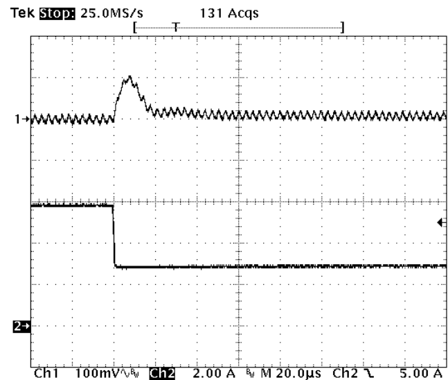
Fig-2.0V-7: Output voltage response for V_{out}=2.0V to negative load current step change from 6A to 3A with slew rate of -5A/\mu s at V_{in}=12V . C_o=47\mu F \times 2 ceramic.
