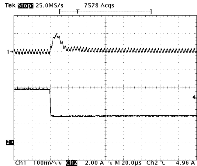
Fig-2.5V-7: Output voltage response for V_{out}=2.5V to negative load current step change from 6A to 3A with slew rate of -5A/us at V_{in}=12V . C_o=47\mu F \times 2 ceramic. Top trace: output voltage (100mV/div.) Bottom trace: load current (2A/div.) Time scale: 20us/div.
