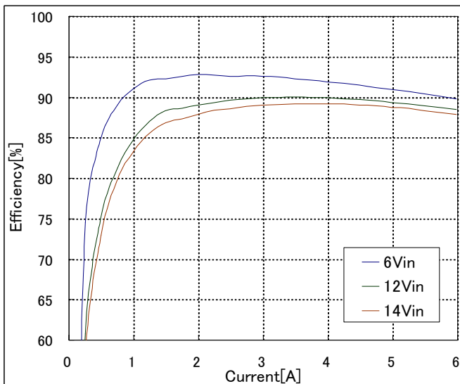
Fig-2.0V-2: Efficiency vs. load current and input voltage for Vout=2.0V. Airflow rate=200 LFM (1m/s) and Ta=25°C.
