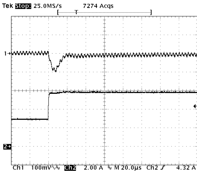
Fig-1.8V-6: Output voltage response for V_{out}=1.8V to positive load current step change from 3A to 6A with slew rate of 5A/\mu s at V_{in}=12V . C_o=47\mu F \times 2 ceramic. Top trace: output voltage (100mV/div.) Bottom trace: load current (2A/div.) Time scale: 20us/div.
