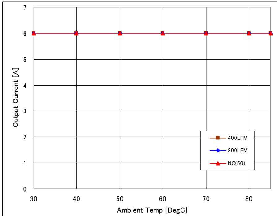
Fig-2.0V-1: Available load current vs. ambient temperature and airflow rates for Vout=2.0V with Vin=12V. Maximum component temperature ≤ 120°C
