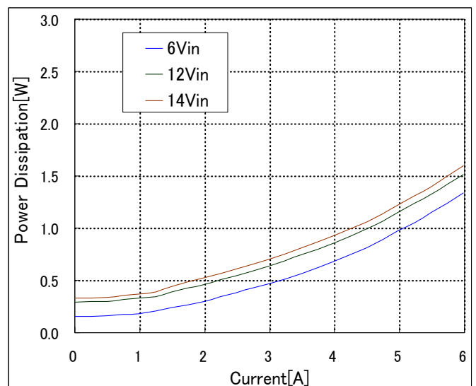
Fig-1.8V-3: Power Loss vs. load current and input voltage for Vout=1.8V. Airflow rate=200 LFM (1m/s) and Ta=25°C.
