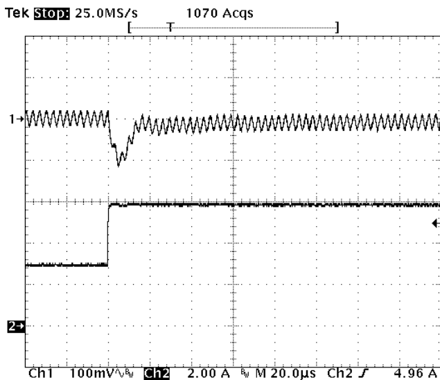
Fig-5.0V-6: Output voltage response for V_{out}=5.0V to positive load current step change from 3A to 6A with slew rate of 5A/\mu s at V_{in}=12V . C_o=47\mu F \times 2 ceramic. Top trace: output voltage (100mV/div.) Bottom trace: load current (2A/div.) Time scale: 20us/div.
