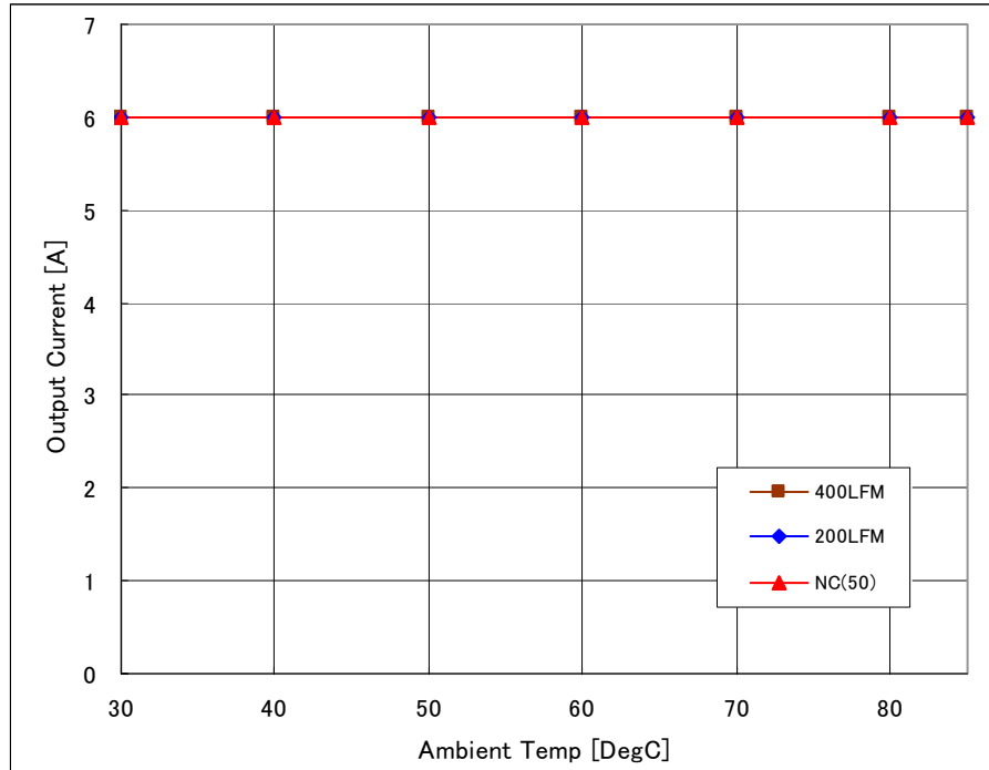
Fig-1.8V-1: Available load current vs. ambient temperature and airflow rates for Vout=1.8V with Vin=12V. Maximum component temperature ≤ 120°C
