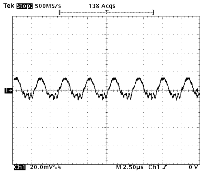
Fig-2.5V-5: Output voltage ripple (20mV/div.) for V_{out}=2.5V at full rated load current into a resistive load with external capacitance 47\mu F \times 2 ceramic + 1uF ceramic at V_{in}=12V . Time scale: 2.5 us/div.
