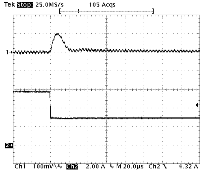
Fig-1.0V-7: Output voltage response for V_{out}=1.0V to negative load current step change from 6A to 3A with slew rate of -5A/\mu s at V_{in}=12V . C_o=47\mu F \times 2 ceramic. Top trace: output voltage (100mV/div.) Bottom trace: load current (2A/div.) Time scale: 20us/div.
