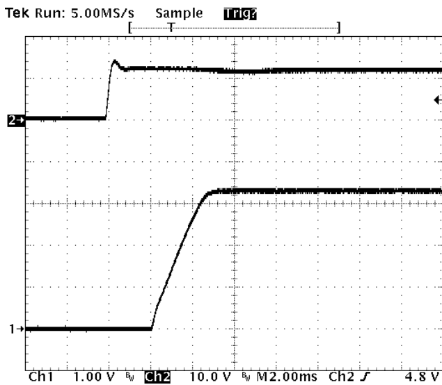
Fig-3.3V-4: Turn-on transient for V_{out}=3.3V with application of V_{in} at full rated load current (resistive) and 47\mu F \times 2 external capacitance at V_{in}=12V .
