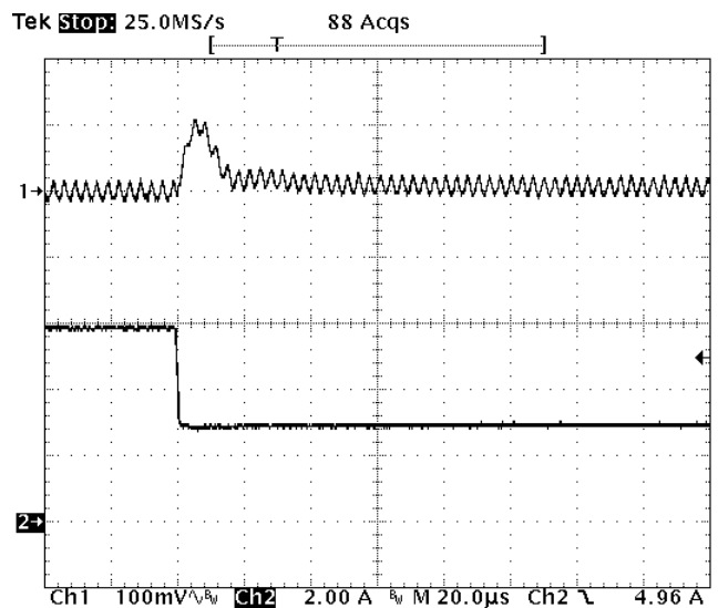
Fig-3.3V-7: Output voltage response for V_{out}=3.3V to negative load current step change from 6A to 3A with slew rate of -5A/\mu s at V_{in}=12V . C_o=47\mu F \times 2 ceramic.
