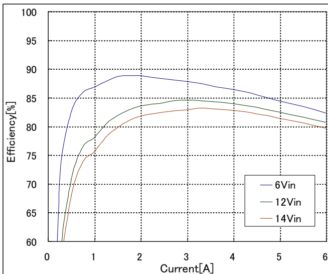
Fig-1.0V-2: Efficiency vs. load current and input voltage for V_{out}=1.0V . Airflow rate=200 LFM (1m/s) and T_a=25^{\circ}C .
