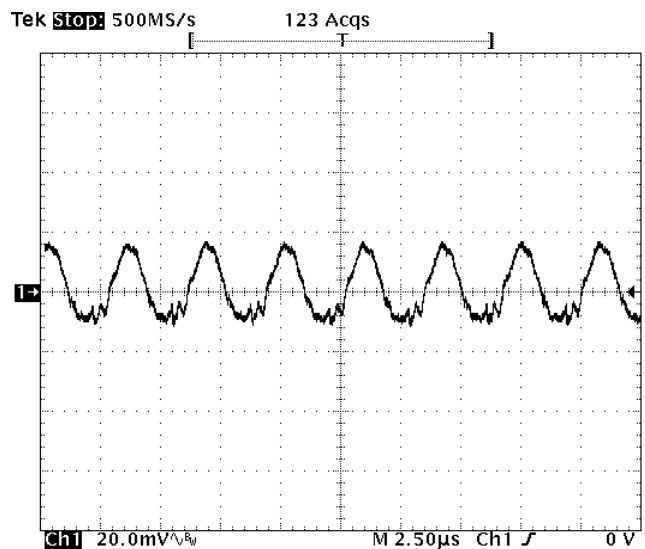
Fig-3.3V-5: Output voltage ripple (20mV/div.) for V_{out}=3.3V at full rated load current into a resistive load with external capacitance 47\mu F \times 2 ceramic + 1\mu F ceramic at V_{in}=12V .
