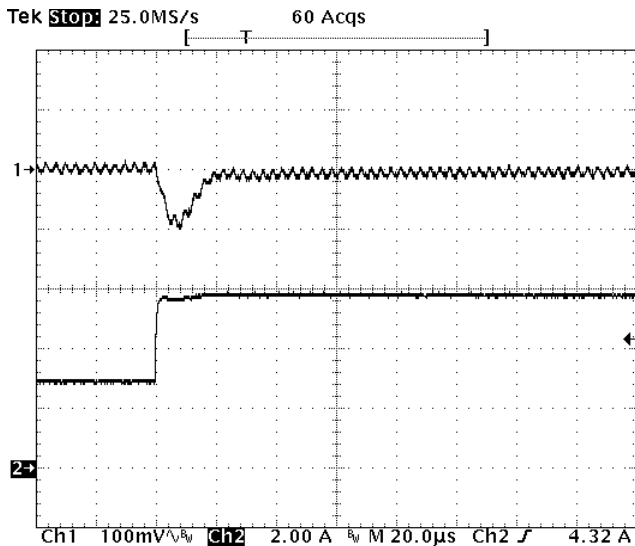
Fig-1.5V-6: Output voltage response for V_{out}=1.5V to positive load current step change from 3A to 6A with slew rate of 5A/\mu s at V_{in}=12V . C_o=47\mu F \times 2 ceramic. Top trace: output voltage (100mV/div.) Bottom trace: load current (2A/div.) Time scale: 20us/div.
