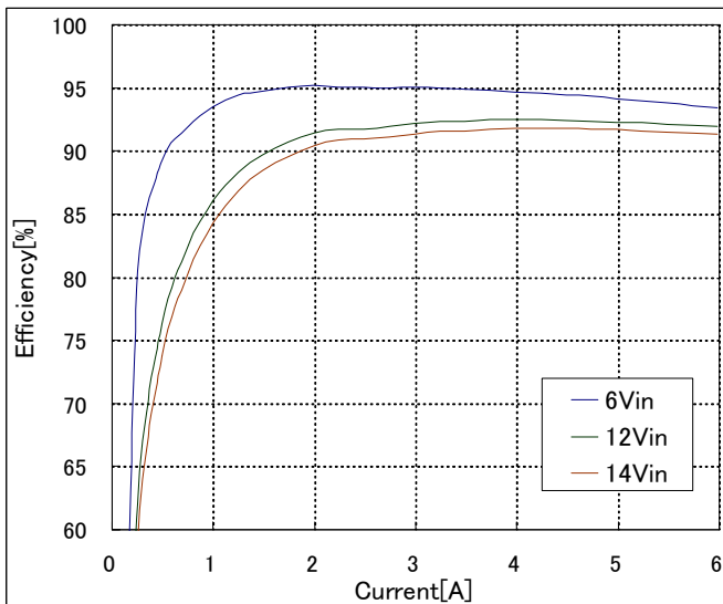
Fig-3.3V-2: Efficiency vs. load current and input voltage for Vout=3.3V. Airflow rate=200 LFM (1m/s) and Ta=25°C.
