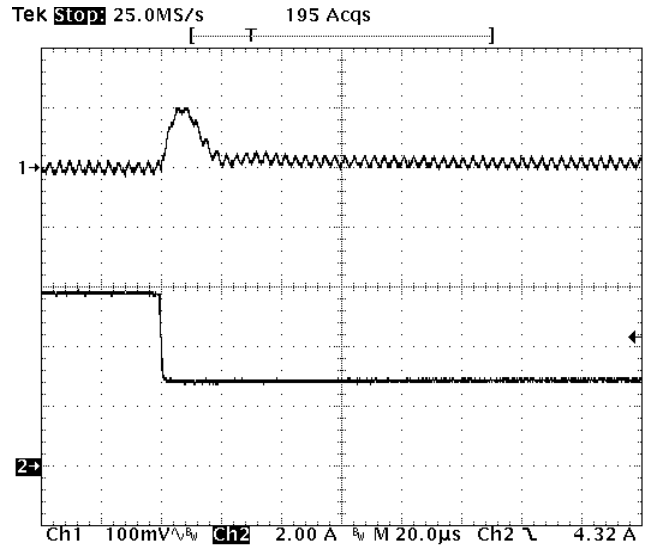
Fig-1.8V-7: Output voltage response for V_{out}=1.8V to negative load current step change from 6A to 3A with slew rate of -5A/\mu s at V_{in}=12V . C_o=47\mu F \times 2 ceramic. Top trace: output voltage (100mV/div.) Bottom trace: load current (2A/div.) Time scale: 20us/div.
