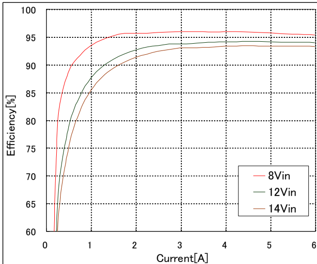
Fig-5.0V-2: Efficiency vs. load current and input voltage for Vout=5.0V. Airflow rate=200 LFM (1m/s) and Ta=25°C.
