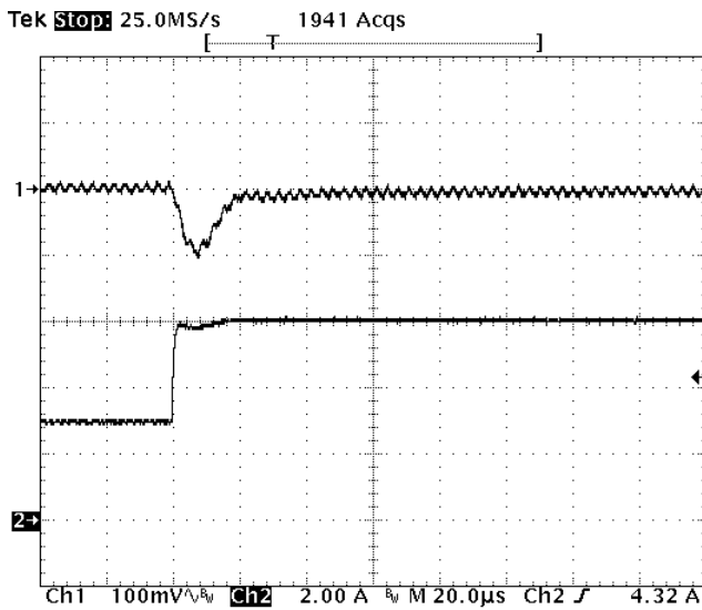
Fig-1.2V-6: Output voltage response for V_{out}=1.2V to positive load current step change from 3A to 6A with slew rate of 5A/us at V_{in}=12V . C_o=47\mu F \times 2 ceramic. Top trace: output voltage (100mV/div.) Bottom trace: load current (2A/div.) Time scale: 20us/div.
