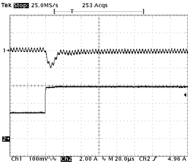
Fig-2.5V-6: Output voltage response for V_{out}=2.5V to positive load current step change from 3A to 6A with slew rate of 5A/us at V_{in}=12V . C_o=47\mu F \times 2 ceramic. Top trace: output voltage (100mV/div.) Bottom trace: load current (2A/div.) Time scale: 20us/div.
