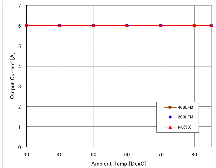
Fig-1.5V-1: Available load current vs. ambient temperature and airflow rates for Vout=1.5V with Vin=12V. Maximum component temperature ≤ 120°C
