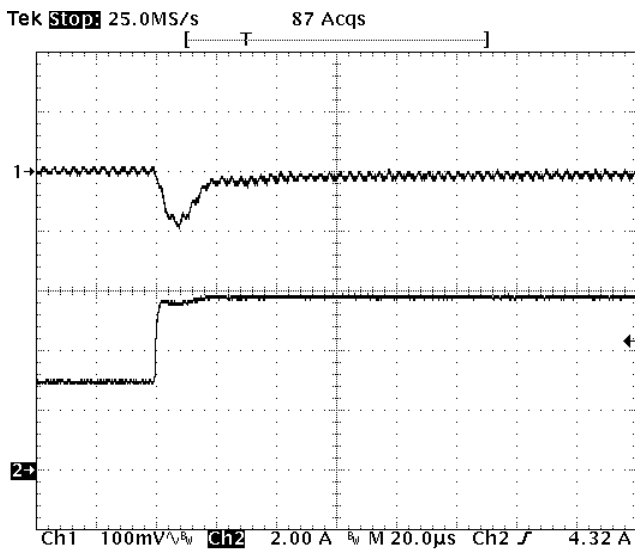
Fig-1.0V-6: Output voltage response for V_{out}=1.0V to positive load current step change from 3A to 6A with slew rate of 5A/\mu s at V_{in}=12V . C_o=47\mu F \times 2 ceramic. Top trace: output voltage (100mV/div.) Bottom trace: load current (2A/div.) Time scale: 20us/div.
