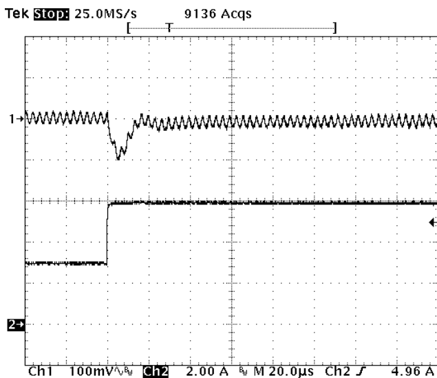
Fig-3.3V-6: Output voltage response for V_{out}=3.3V to positive load current step change from 3A to 6A with slew rate of 5A/\mu s at V_{in}=12V . C_o=47\mu F \times 2 ceramic.
