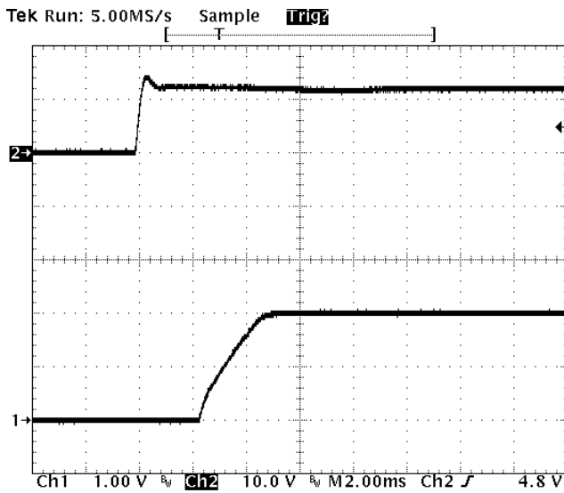
Fig-2.0V-4: Turn-on transient for V_{out}=2.0V with application of V_{in} at full rated load current (resistive) and 47\mu F \times 2 external capacitance at V_{in}=12V .
