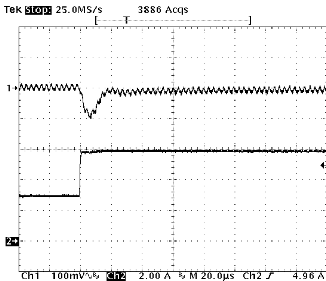
Fig-2.0V-6: Output voltage response for V_{out}=2.0V to positive load current step change from 3A to 6A with slew rate of 5A/\mu s at V_{in}=12V . C_o=47\mu F \times 2 ceramic.
