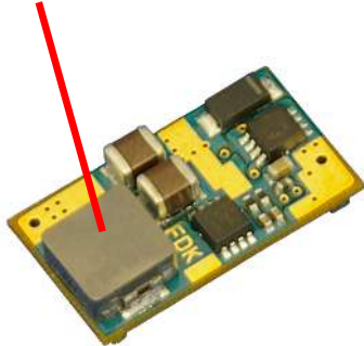
Fig. C: Location of the thermocouples for thermal testing
