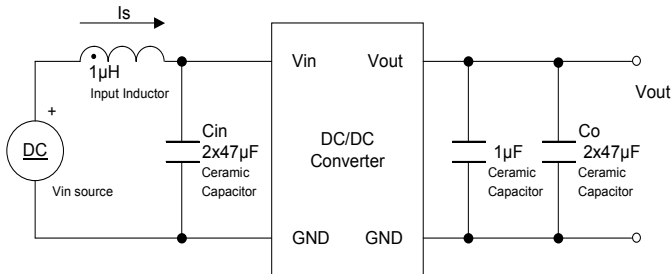
Fig. D: Test setup for measuring output voltage ripple & input reflected ripple current
