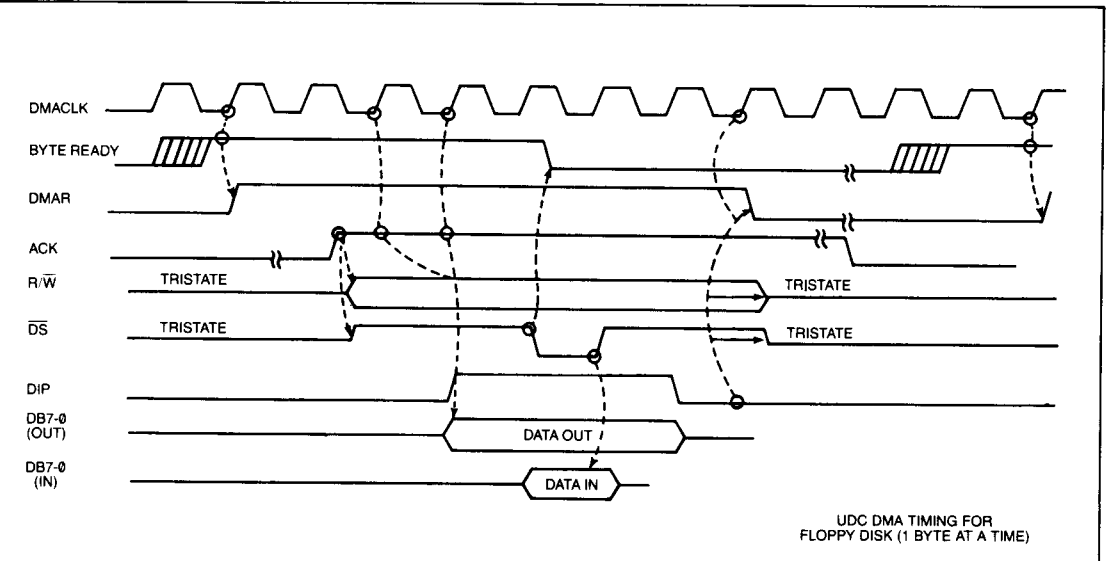
FIGURE 6: UDC DMA TIMING FOR FLOPPY DISK (1 BYTE AT A TIME)
