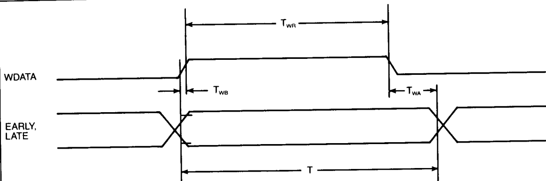
FIGURE 8: UDC DATA WRITE TIMING
