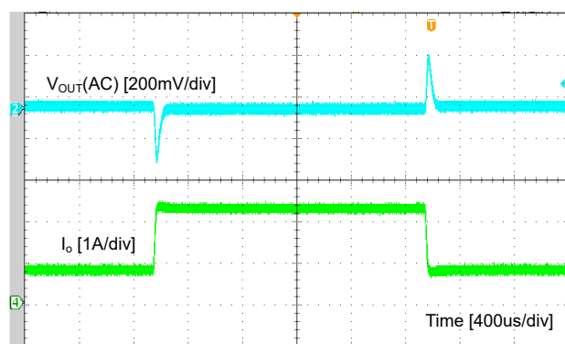
Figure 9-6. Load Transient
