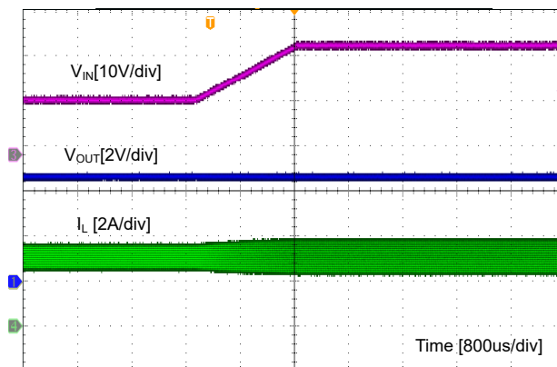
Figure 9-7. Line Transient
