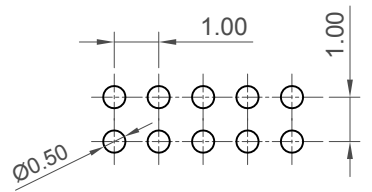
Recommended PCB Layout General TOL: ±0.05
