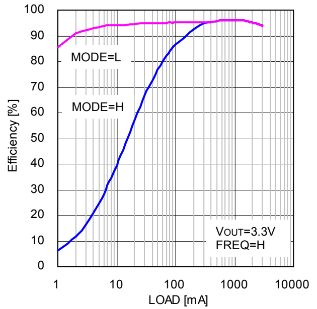
Figure 9. Efficiency vs Load Current (VIN=5V, VOUT=3.3V, L=1.5µH, FREQ=H)
