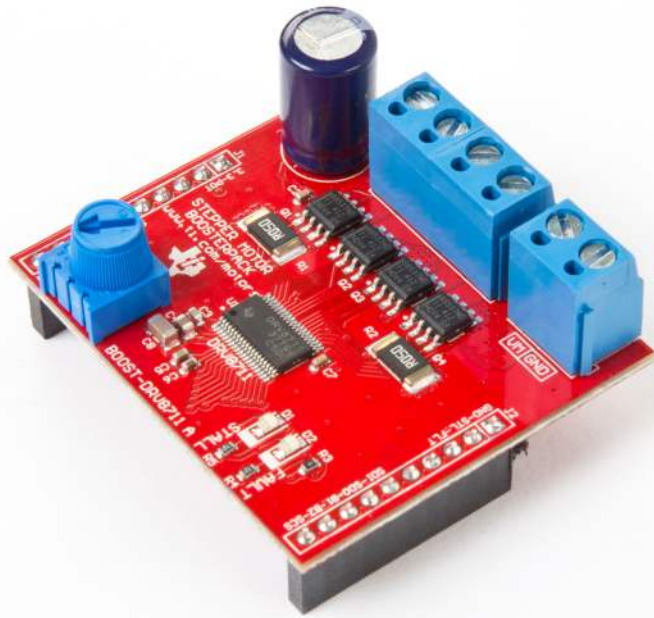
Figure 1. BOOST-DRV8711 Stand-Alone
