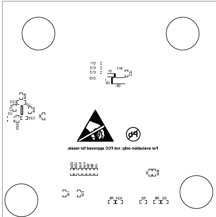
Figure 17. Bottom Assembly
