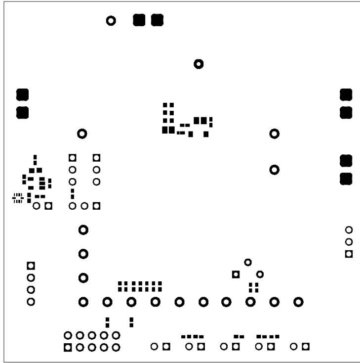
Figure 16. Bottom Solder
