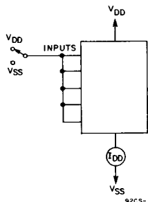
Fig. 10 – Quiescent device current test circuit.
