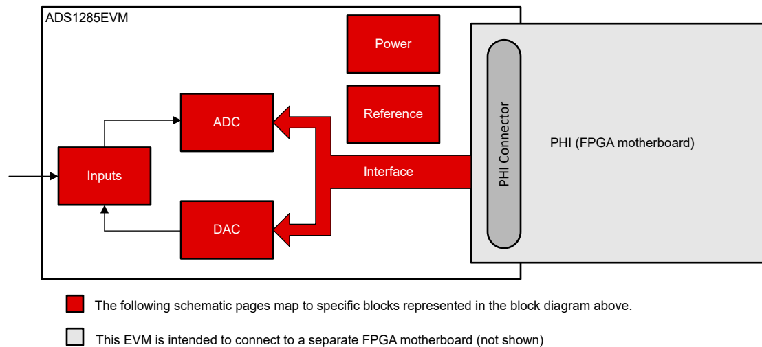
Figure 9-7. ADS1285EVM-PDK Block Diagram
