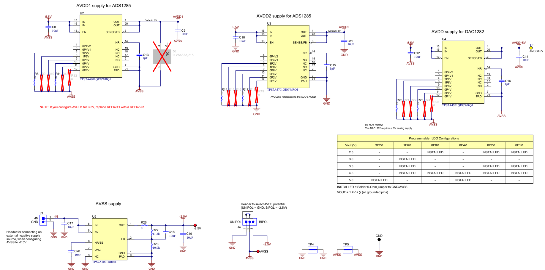
Figure 9-11. ADS1285EVM-PDK Power-Supply Schematic
