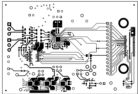
Figure 9-2. Top Layer
