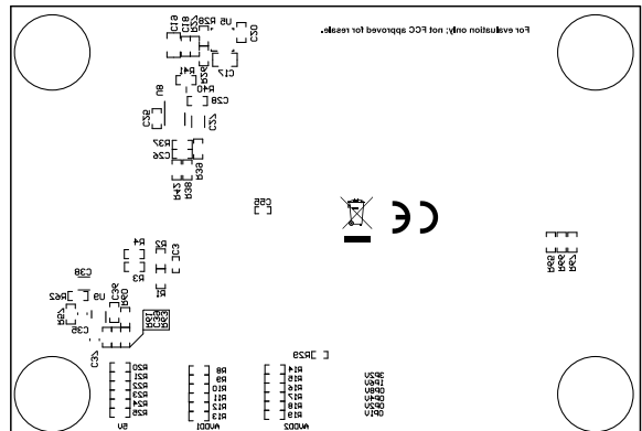
Figure 9-6. Bottom Silkscreen
