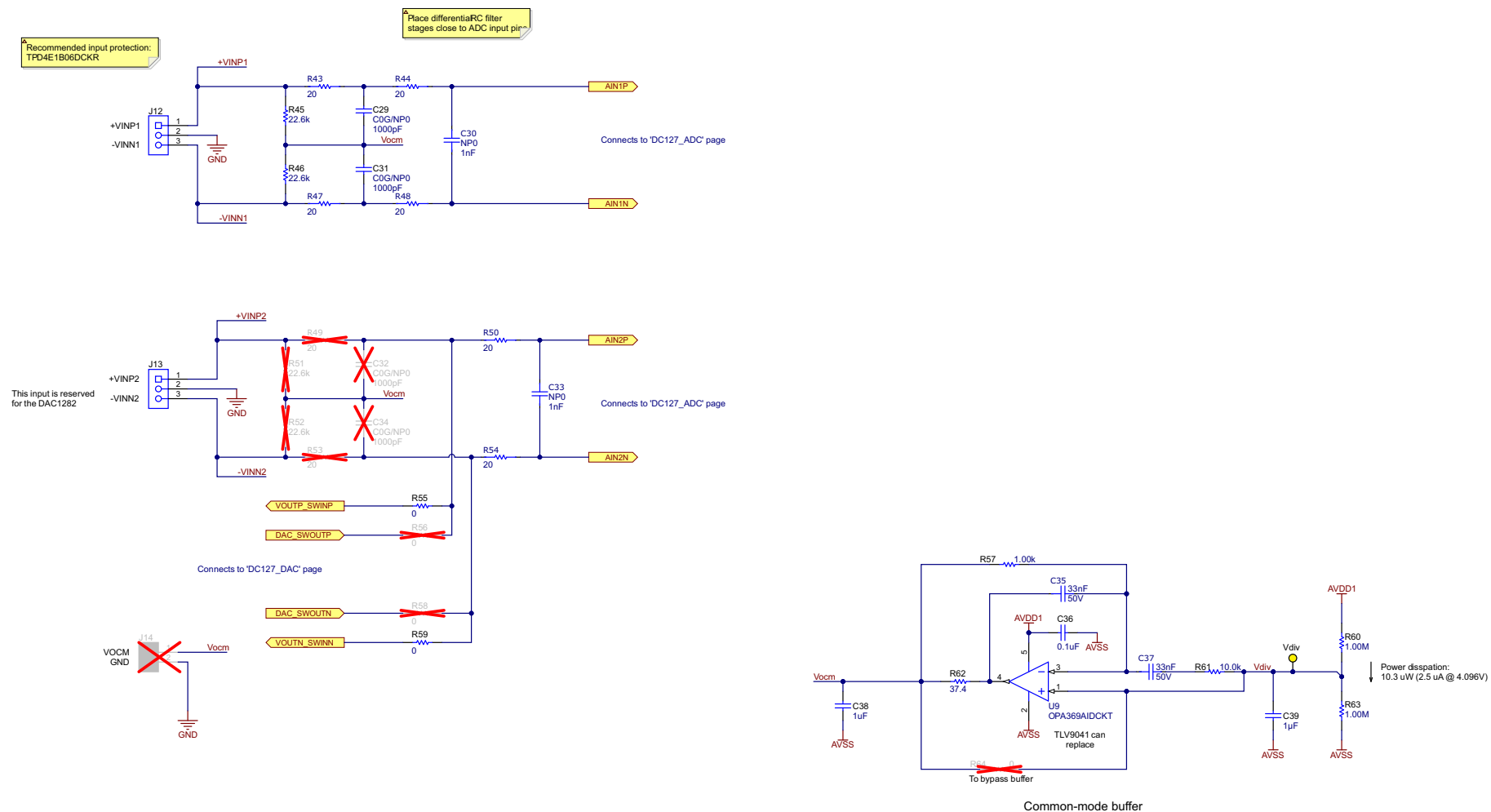
Figure 9-9. ADS1285EVM-PDK Analog Inputs and Common-Mode Buffer Schematic
