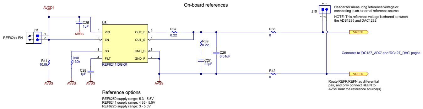
Figure 5-3. Voltage Reference (Schematic)
