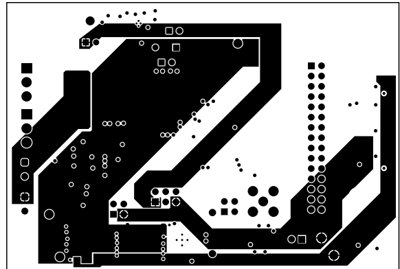
Figure 9-4. Power Layer
