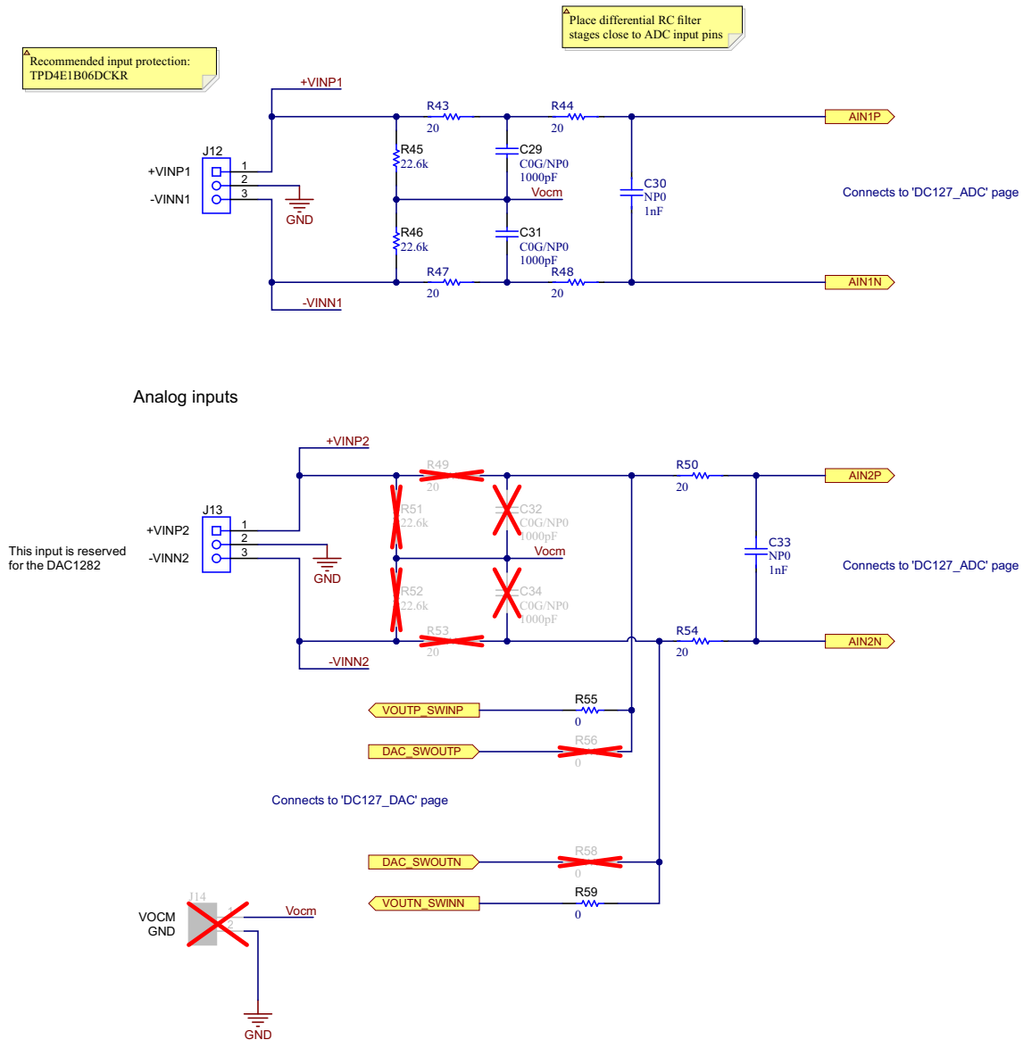
Figure 3-1. Input Terminal Blocks and Headers (Schematic)
