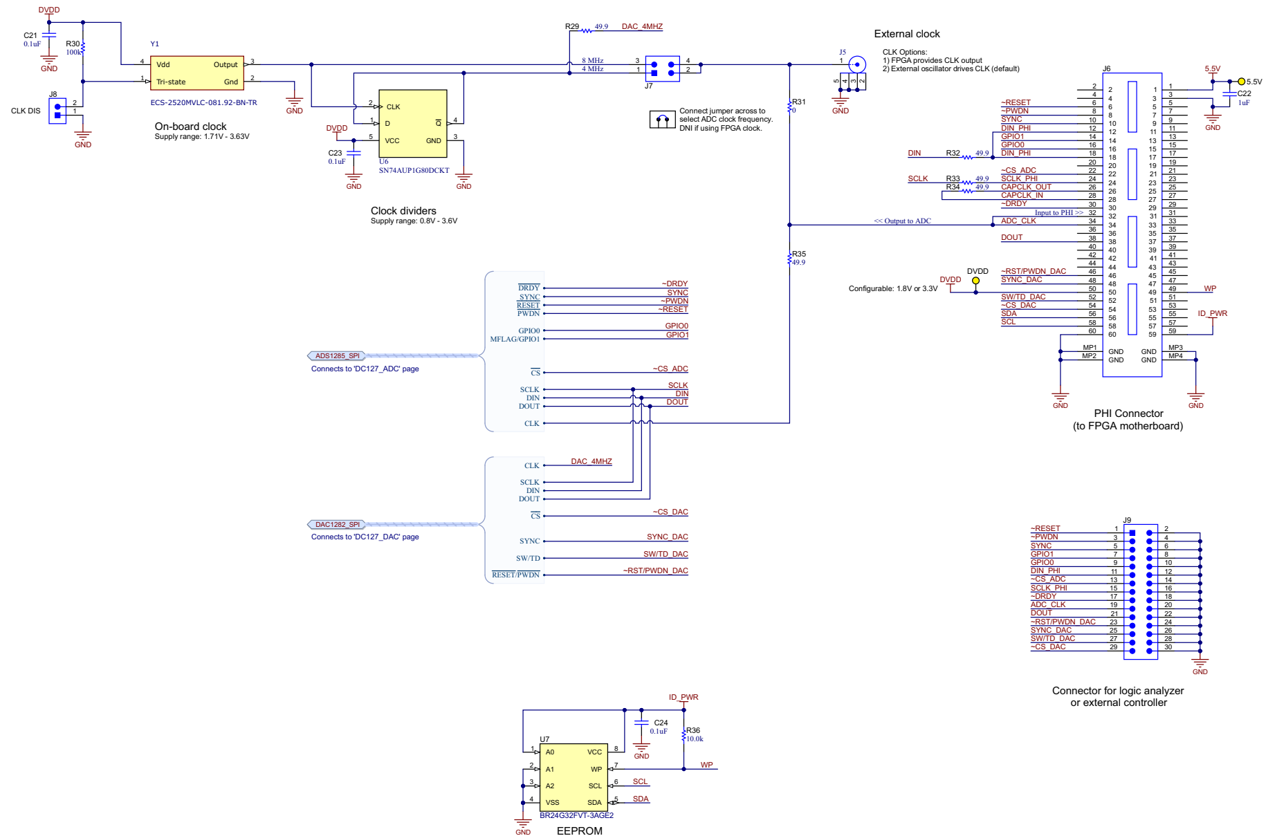
Figure 9-10. ADS1285EVM-PDK Clock and Interface Schematic
