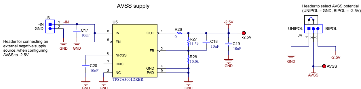
Figure 5-2. ADS1285EVM-PDK Unipolar and Bidirectional Supplies Selection (Schematic)
