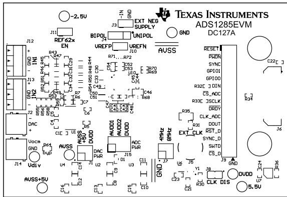
Figure 9-1. Top Silkscreen
