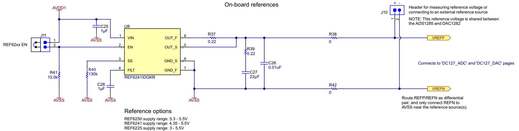
Figure 9-12. ADS1285EVM-PDK Reference Voltage Schematic
