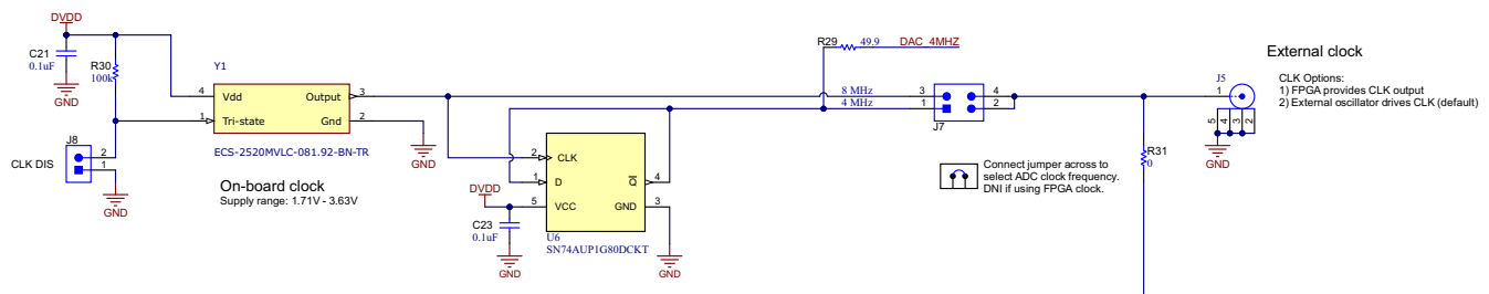
Figure 3-2. CLK Source (Schematic)
