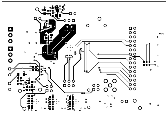
Figure 9-5. Bottom Layer
