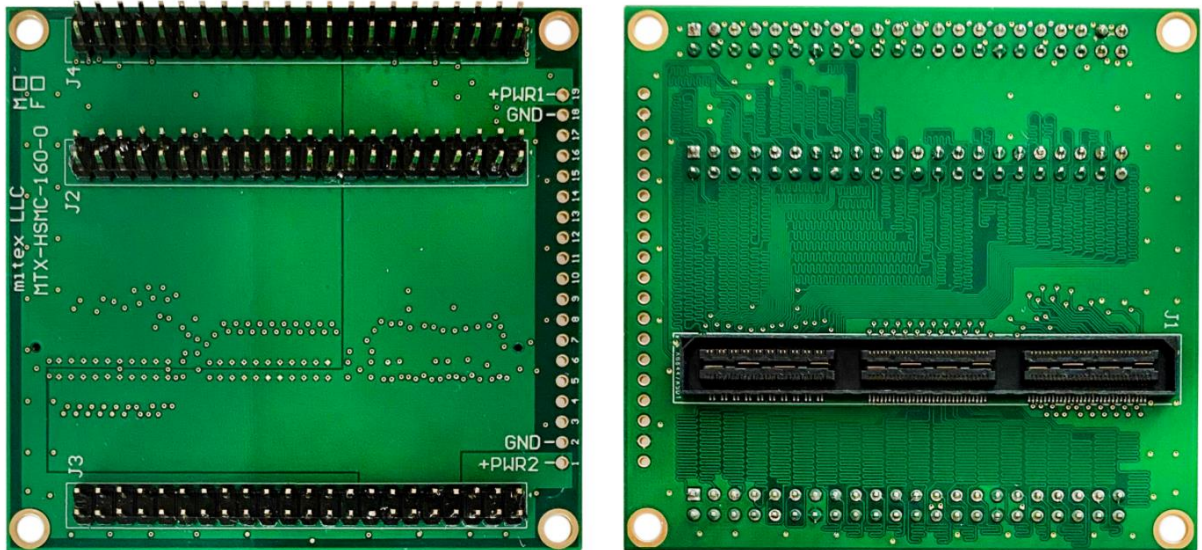
Figure 1. MTX-HSMC-160-0 board top and back side view. Female version.
