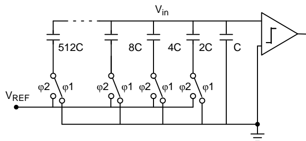
Figure 17. The Conversion Phase of the Typical ADC
