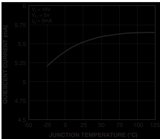
Figure 3. Quiescent Current
