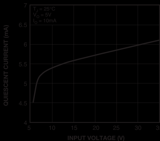
Figure 6. Quiescent Current
