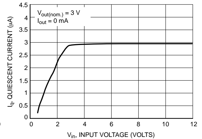
Figure 6. Quiescent Current versus Input Voltage
