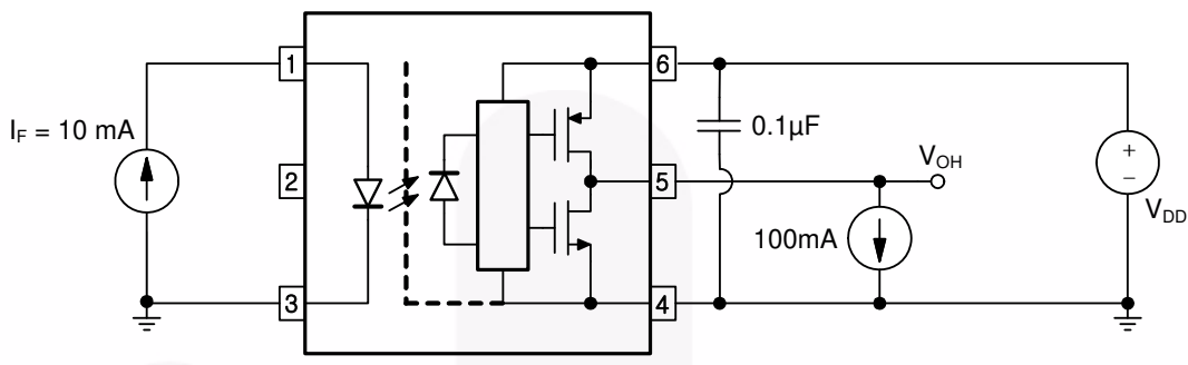
Figure 25. V_{OH} Test Circuit
