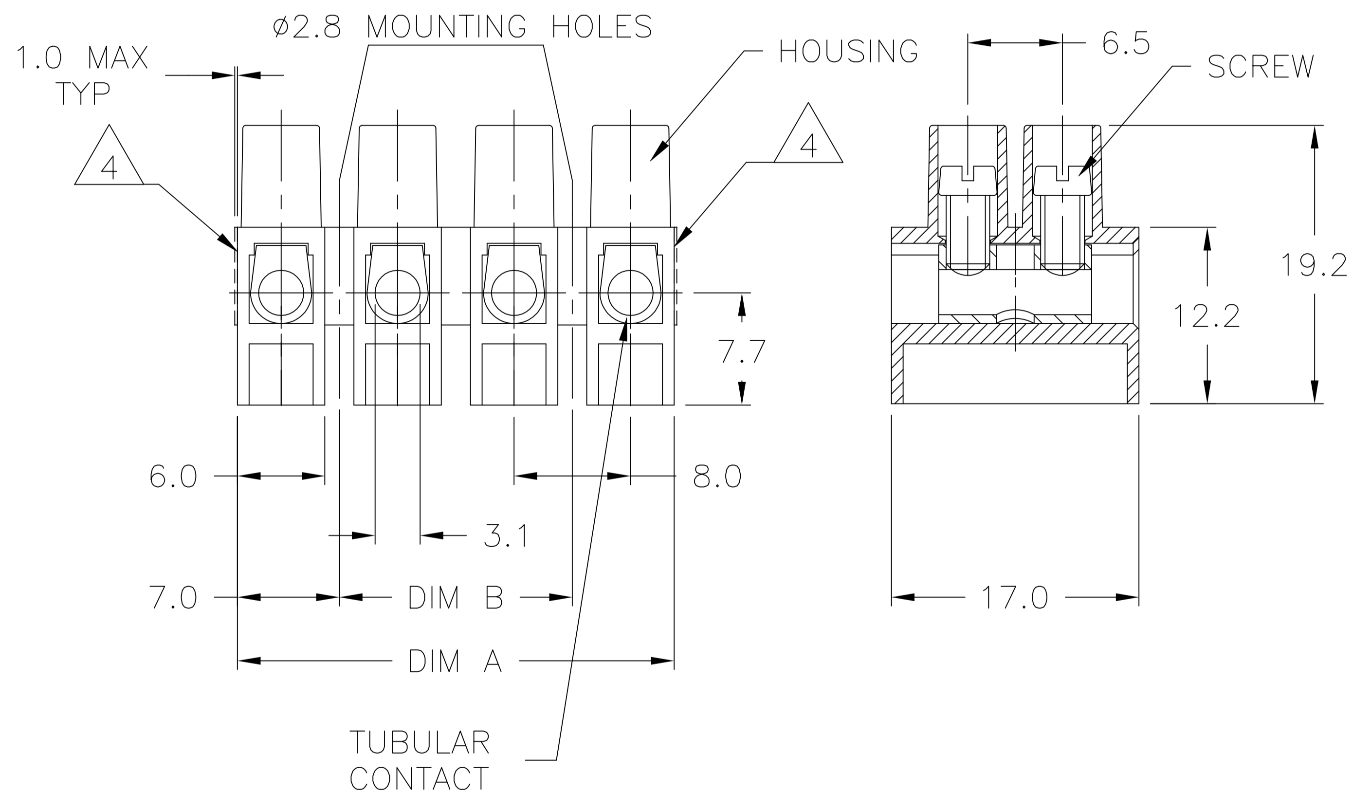
1776321-4 AS SHOWN
