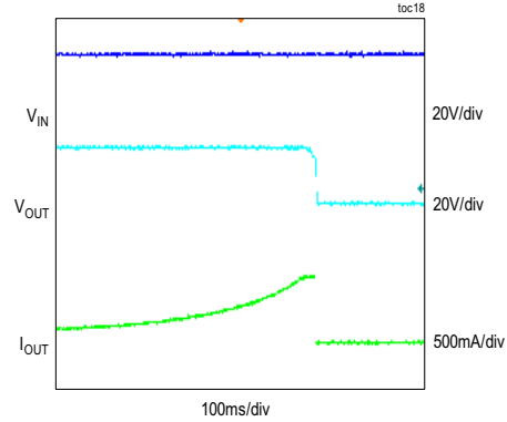
CURRENT-LIMIT RESPONSE
