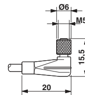
Dimensioned drawing
