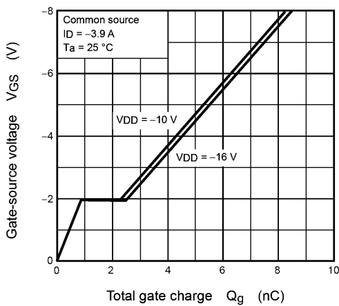
Fig. 8.11 Dynamic Input/Output Characteristics
