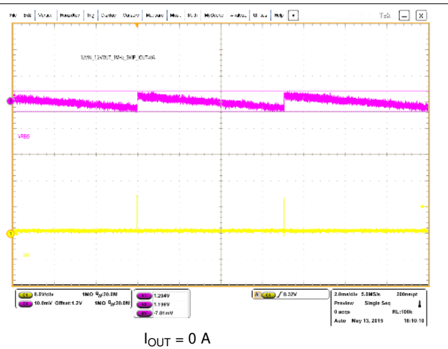
Figure 44. Auto-skip Mode Steady-State Operation
