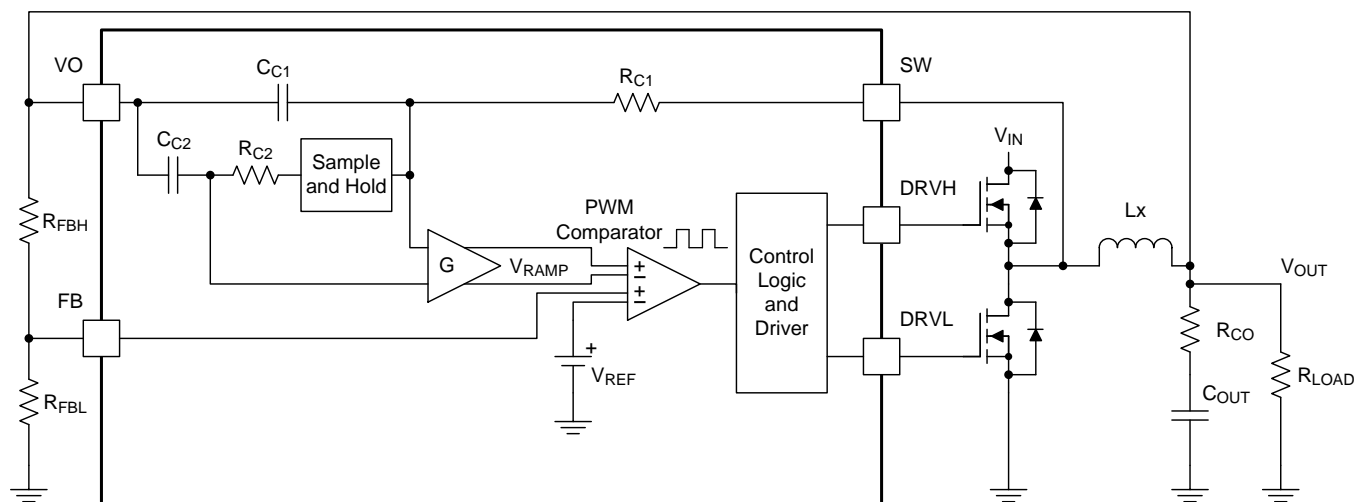
Figure 32. D-CAP3 Mode
