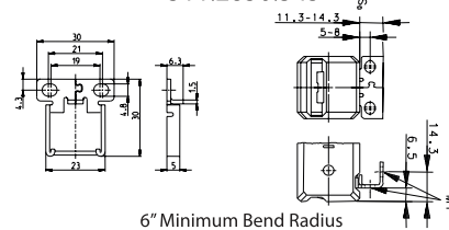
M2 ACTUATOR KEY 311.2850.345
