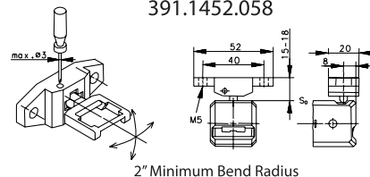
MRU ACTUATOR KEY 391.1452.058
