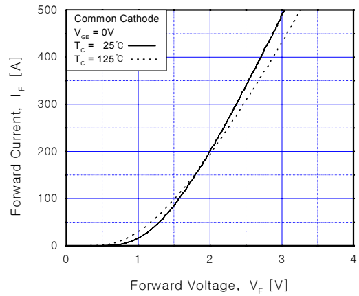
Fig 12. Forward Characteristics (diode)
