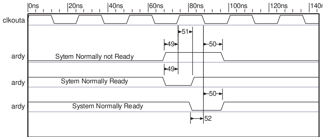
Figure 23. ardy—Asynchronous Ready
