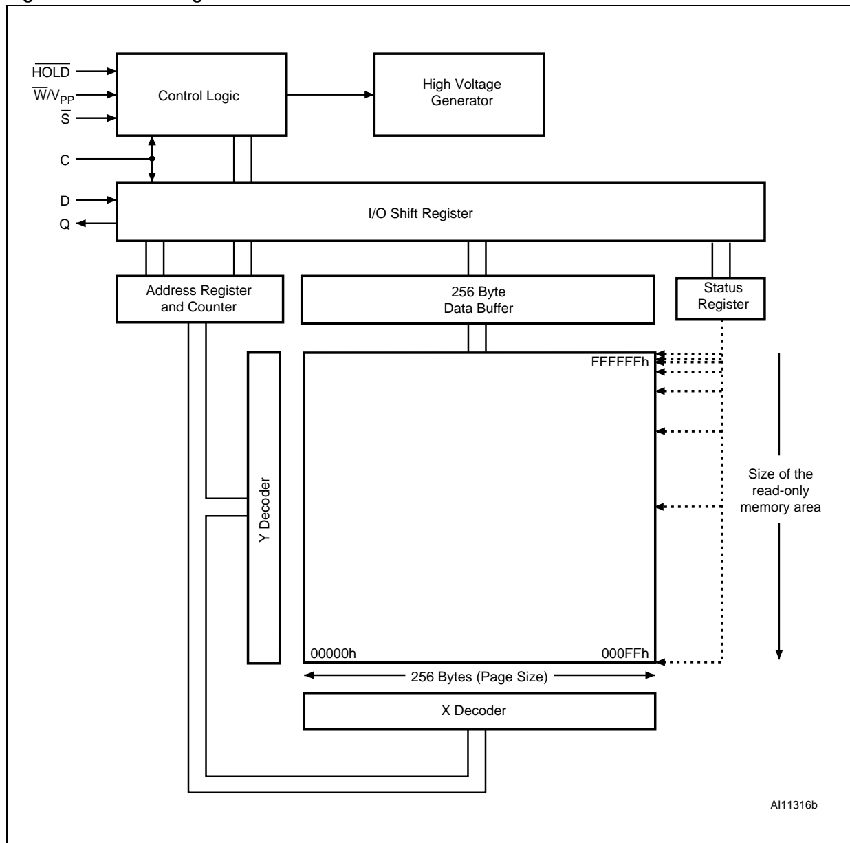
Figure 7. Block diagram
