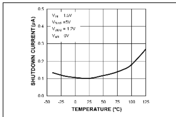
FIGURE 2-19: V_{IN} Shutdown Current vs. Temperature.
