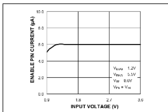
FIGURE 2-8: Enable Pin Current vs. Input Voltage.
