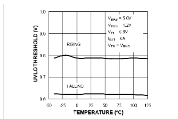
FIGURE 2-20: V_{IN} UVLO Threshold vs. Temperature.
