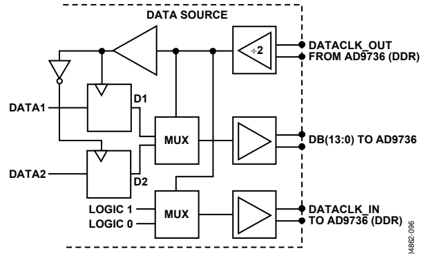
Figure 98. Recommended FPGA/ASIC Configuration for Driving AD9736 Digital Inputs, 2x Mode
