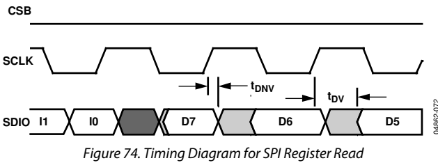
Figure 74. Timing Diagram for SPI Register Read
