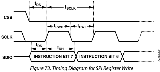
Figure 73. Timing Diagram for SPI Register Write
