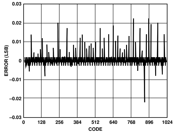
Figure 37. AD9734 DNL, 25°C, 20 mA FS
