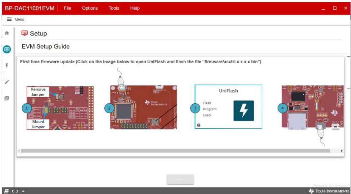
Figure 11. Setup Page
