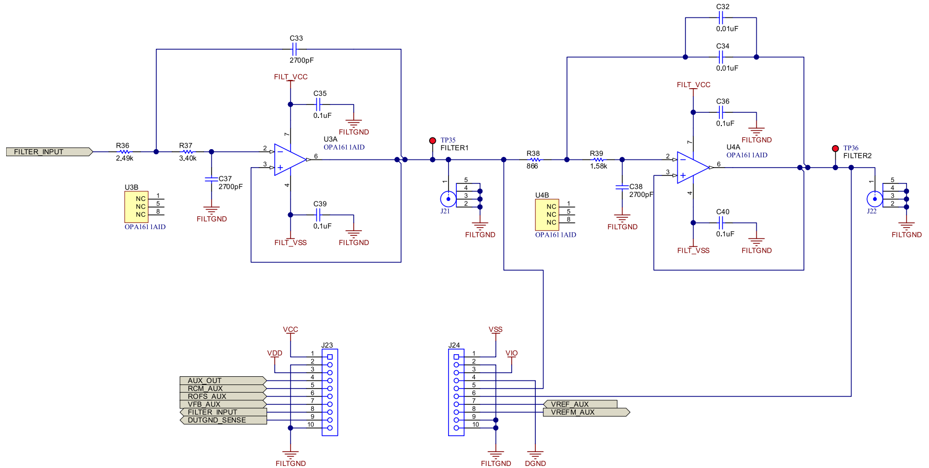
Figure 18. Schematic Page 3
