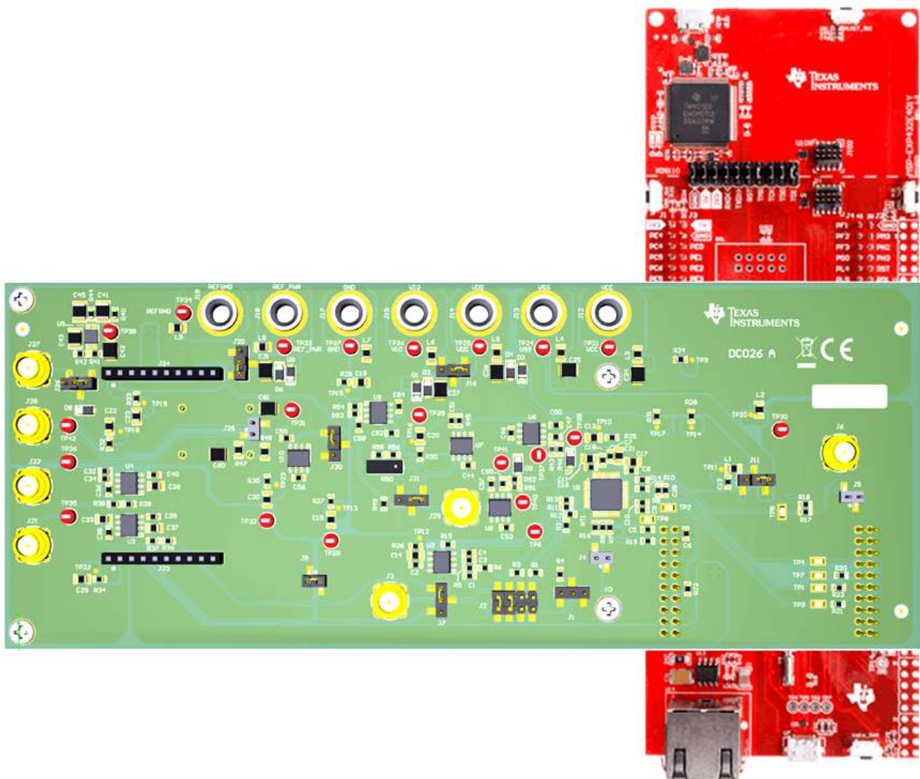
Figure 5. Hardware Setup
