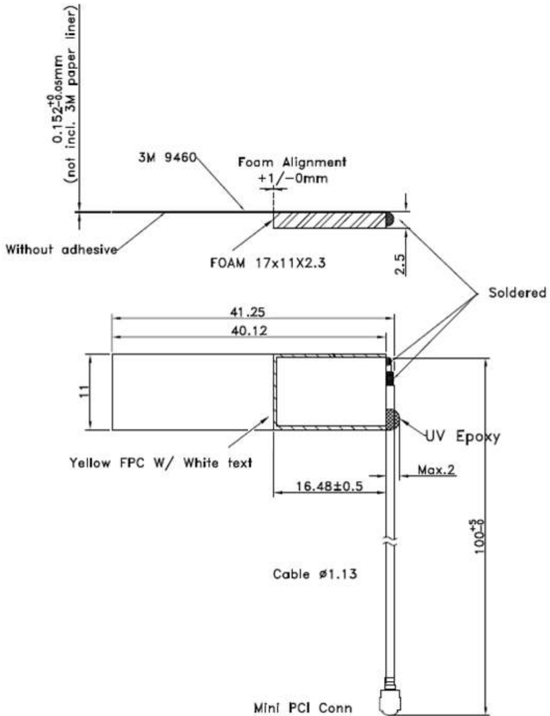
Figure 1 Physical Dimensions
