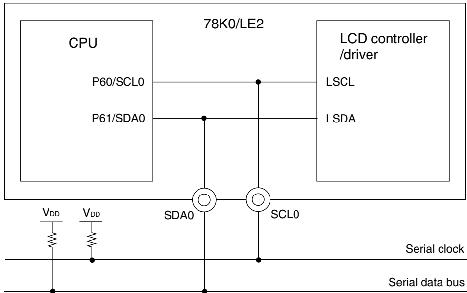
Figure 16-29. System configuration
