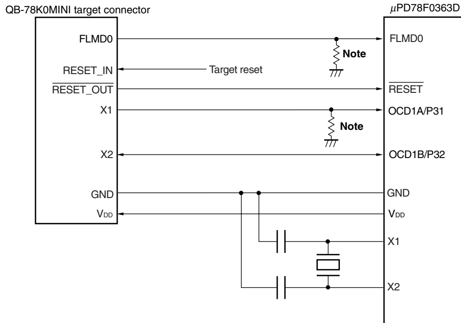
Figure 25-2. Connection Example of QB-78K0MINI and \mu PD78F0363D (When OCD1A and OCD1B Are Used)
