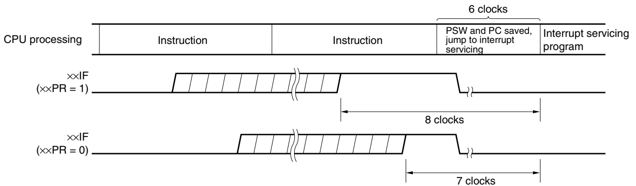
Figure 18-8. Interrupt Request Acknowledgement Timing (Minimum Time)
