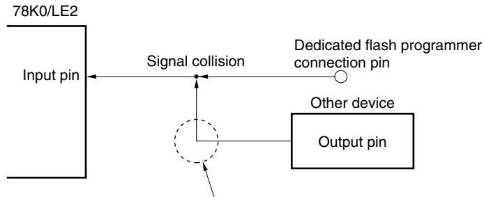
Figure 24-8. Signal Collision (Input Pin of Serial Interface)
