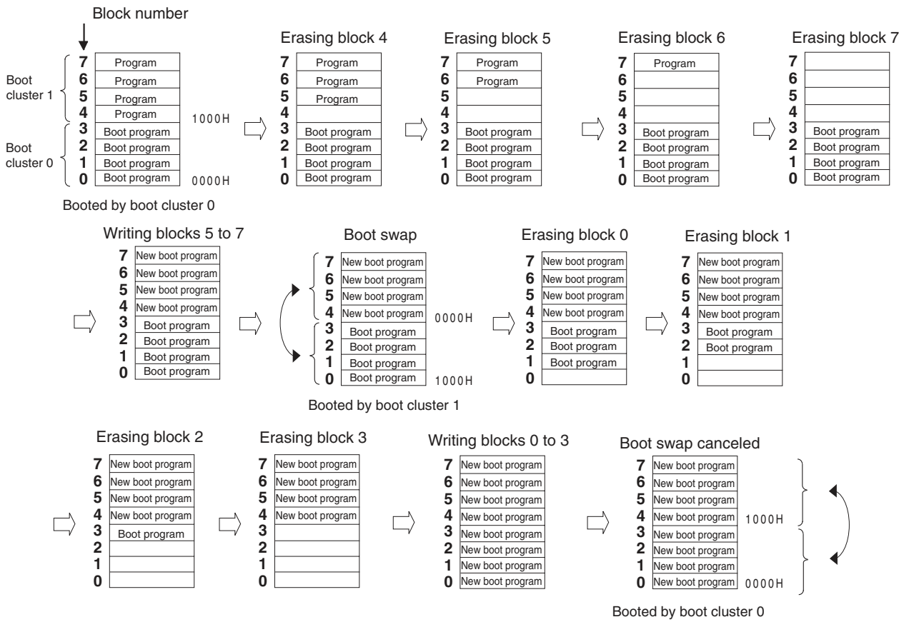
Figure 24-16. Example of Executing Boot Swapping
