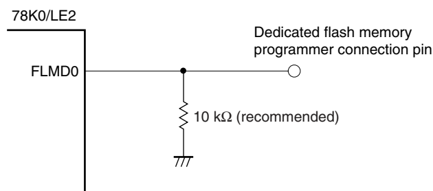
Figure 24-7. FLMD0 Pin Connection Example
