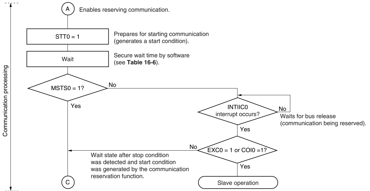
Figure 16-24. Master Operation Flowchart (Multi-Master System) (2/3)
