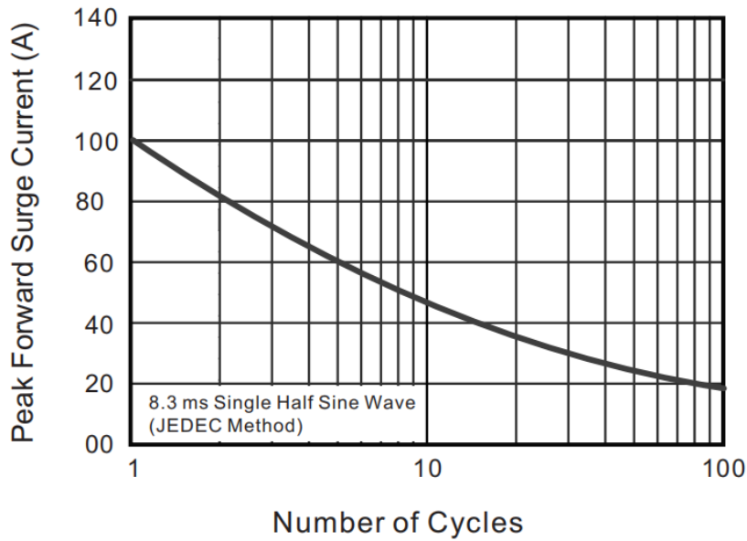
Fig.6 Maximum Non-Repetitive Peak Forward Surge Current
