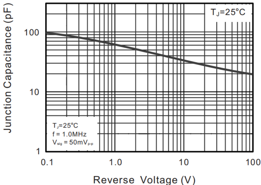
Fig.5 Typical Junction Capacitance
