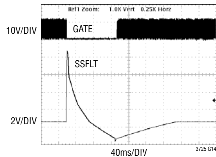
Fault Operation
