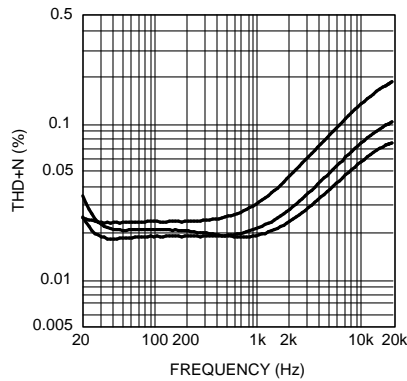
Figure 16. Stereo THD+N vs Frequency R_L = 16\Omega , A_v = 0\text{dB} at (from left to bottom at 10kHz): V_{DD} = 2\text{V} , P_{OUT} = 7\text{mW} ; V_{DD} = 3\text{V} , P_{OUT} = 36\text{mW} ; V_{DD} = 4\text{V} , P_{OUT} = 92\text{mW} ; both channels driven and measured
