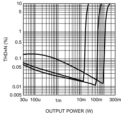
Figure 14. Stereo THD+N vs Output Power R_L = 32\Omega , A_v = 0\text{dB} , f = 1\text{kHz} at (from left to right at 1% THD+N): V_{DD} = 2\text{V} , V_{DD} = 3\text{V} , V_{DD} = 4\text{V} , both channels driven and measured
