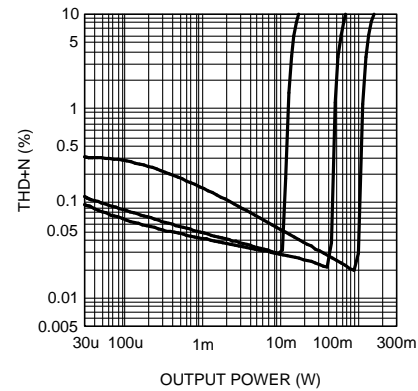
Figure 11. Stereo THD+N vs Output Power R_L = 16\Omega , A_v = 0\text{dB} , f = 1\text{kHz} at (from left to right at 1% THD+N): V_{DD} = 2\text{V} , V_{DD} = 3\text{V} , V_{DD} = 4\text{V} , both channels driven and measured
