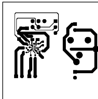
Figure 5. Top Layer (Shown 2.6X actual size)
