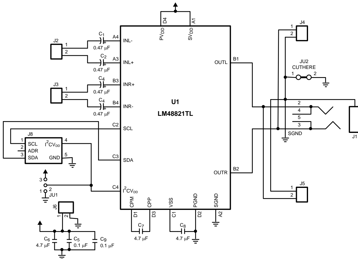
Figure 2. LM48821 Demonstration Board Schematic
