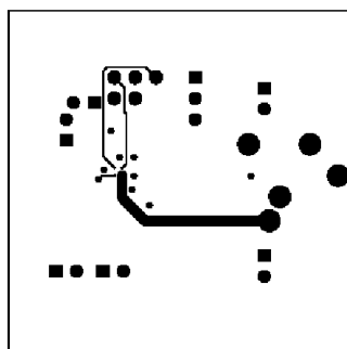
Figure 6. Upper Middle Layer (Shown 2.6X actual size)
