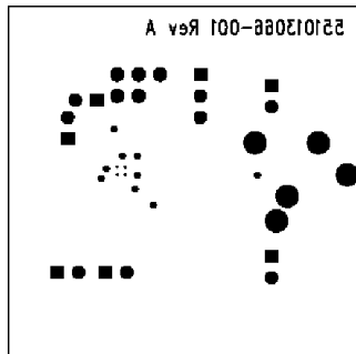
Figure 9. Bottom Silk Layer (Shown 2.6X actual size)
