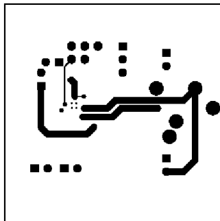
Figure 8. Bottom Layer (Shown 2.6X actual size)
