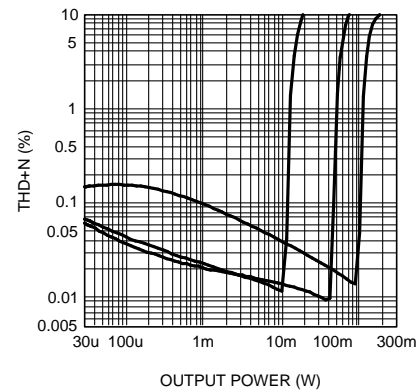
Figure 13. Stereo THD+N vs Output Power R_L = 32\Omega , A_v = 0\text{dB} , f = 100\text{Hz} at (from left to right at 1% THD+N): V_{DD} = 2\text{V} , V_{DD} = 3\text{V} , V_{DD} = 4\text{V} , both channels driven and measured
