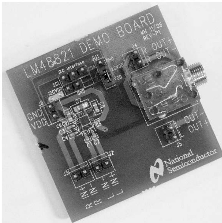
Figure 1. LM48821 Demonstration Board
