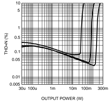
Figure 15. Stereo THD+N vs Output Power R_L = 32\Omega , A_v = 0\text{dB} , f = 10\text{kHz} at (from left to right at 1% THD+N): V_{DD} = 2\text{V} , V_{DD} = 3\text{V} , V_{DD} = 4\text{V} , both channels driven and measured
