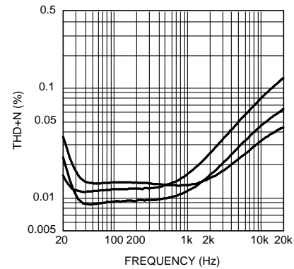
Figure 17. Stereo THD+N vs Frequency R_L = 32\Omega , A_v = 0\text{dB} at (from left to bottom at 10kHz): V_{DD} = 2\text{V} , P_{OUT} = 10\text{mW} ; V_{DD} = 3\text{V} , P_{OUT} = 38\text{mW} ; V_{DD} = 4\text{V} , P_{OUT} = 85\text{mW} ; both channels driven and measured
