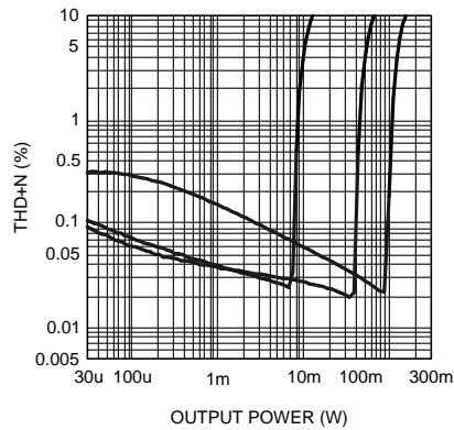
Figure 10. Stereo THD+N vs Output Power R_L = 16\Omega , A_v = 0\text{dB} , f = 100\text{Hz} at (from left to right at 1% THD+N): V_{DD} = 2\text{V} , V_{DD} = 3\text{V} , V_{DD} = 4\text{V} , both channels driven and measured
