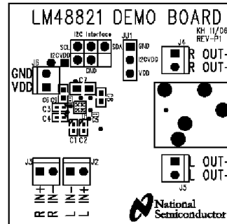
Figure 4. Top Silkscreen (Shown 2.6X actual size)
