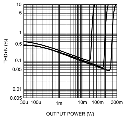
Figure 12. Stereo THD+N vs Output Power R_L = 16\Omega , A_v = 0\text{dB} , f = 10\text{kHz} at (from left to right at 1% THD+N): V_{DD} = 2\text{V} , V_{DD} = 3\text{V} , V_{DD} = 4\text{V} , both channels driven and measured
