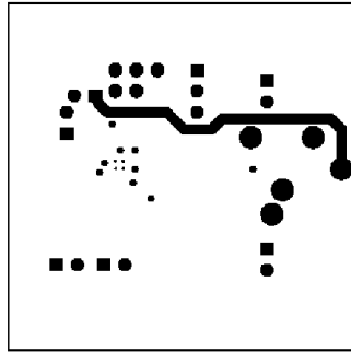
Figure 7. Lower Middle Layer (Shown 2.6X actual size)
