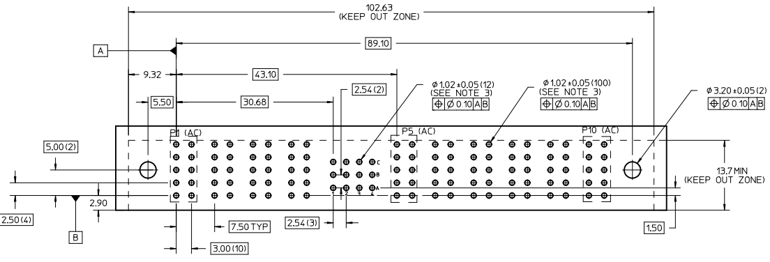
RECOMMENDED PCB LAYOUT AND KEEP-OUT ZONE
