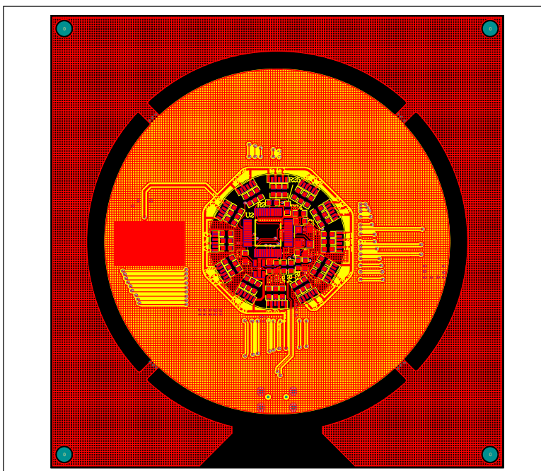
Figure 4: Board PCB Layout - Top Layer
