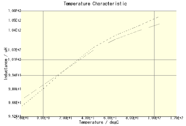
CLF7045T-101M-CA(DC = 0A)
