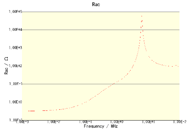
CLF7045T-101M-CA
