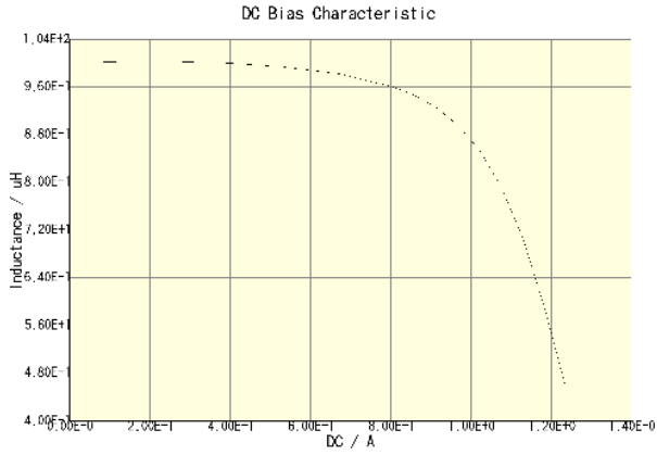
CLF7045T-101M-CA(Amb. Temp. = 20degc)
