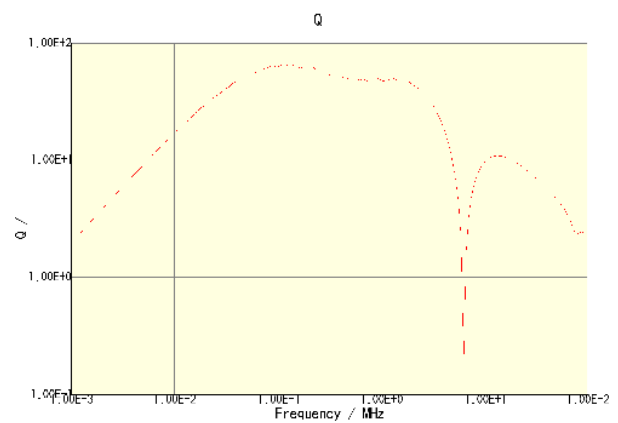
CLF7045T-101M-CA
