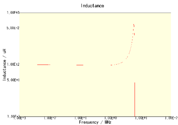
CLF7045T-101M-CA
