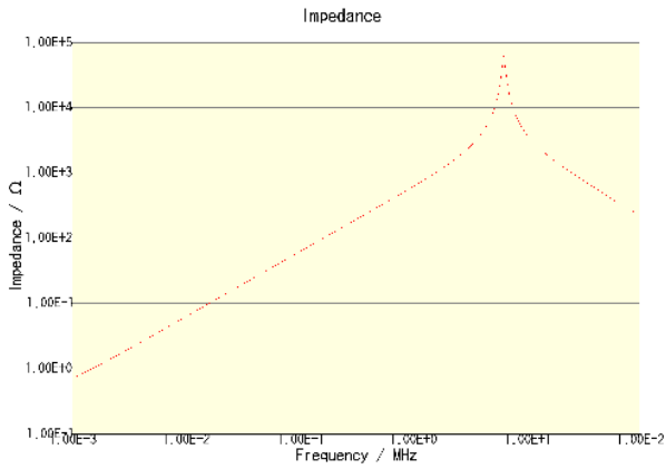
CLF7045T-101M-CA
